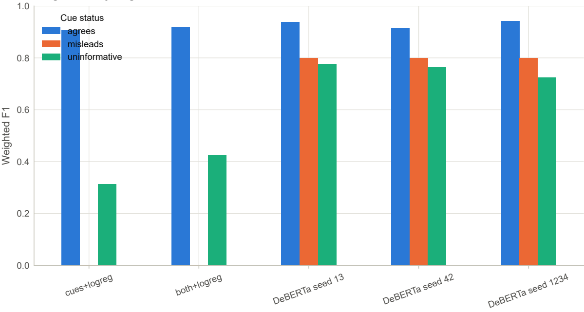
Weighted F1 by length-cue status
