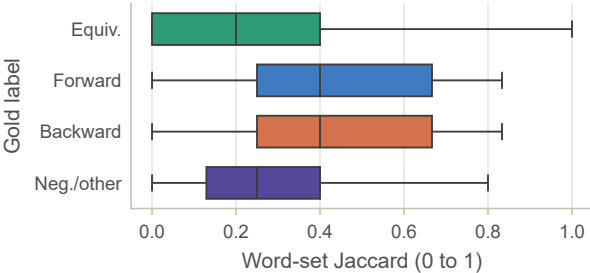
Lexical overlap
