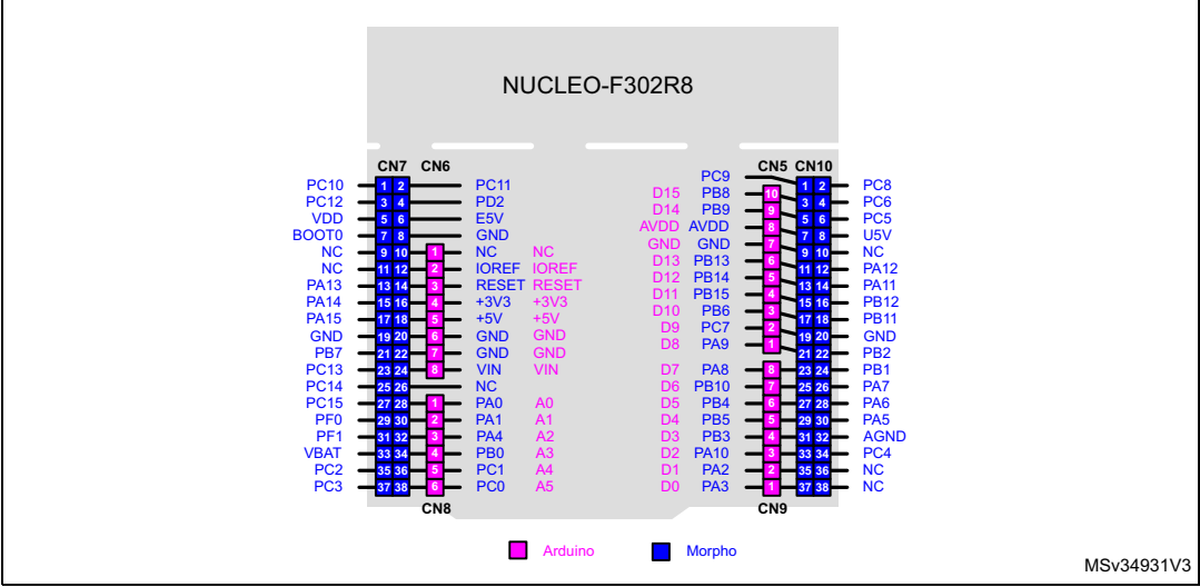
Figure 14. NUCLEO-F302R8
