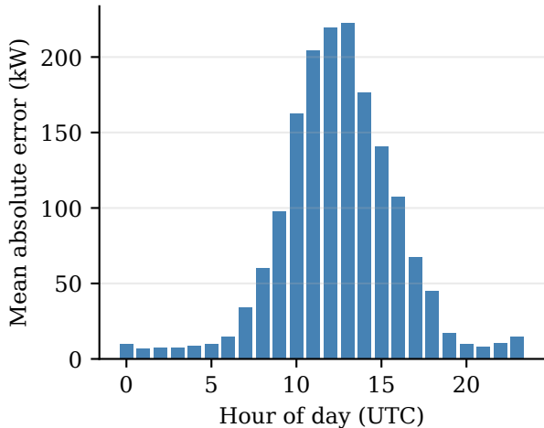
Random day-fold NNLS stacking
