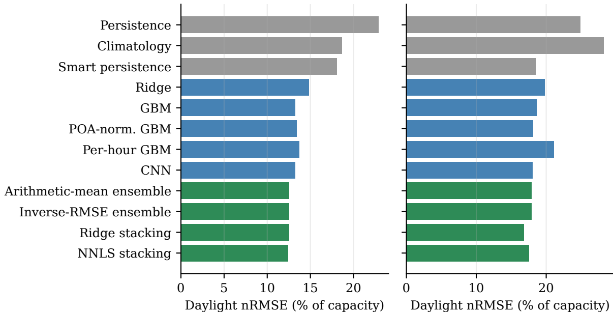
Random day-fold
