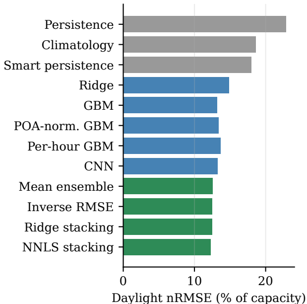
Random day-fold
