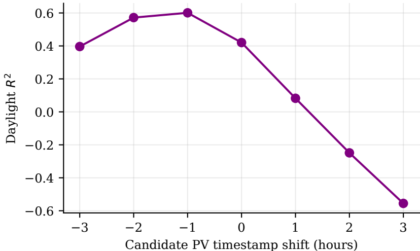
Irradiance-proxy agreement against timestamp shift
