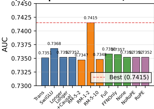
(a) Component Ablation (5000 steps)
