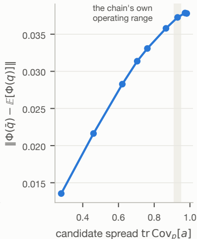
(b) falls as belief sharpens
