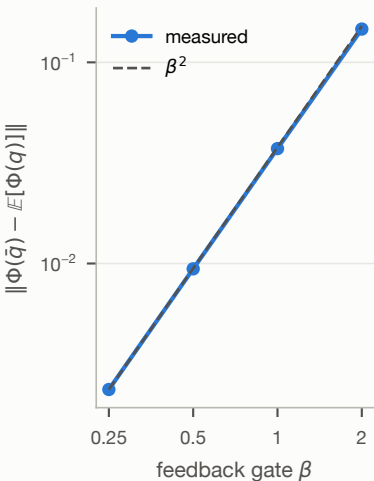
(a) the \beta^2 law
