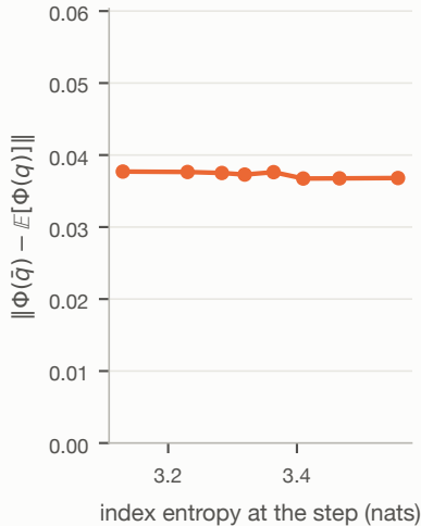
(c) but flat across its own steps
