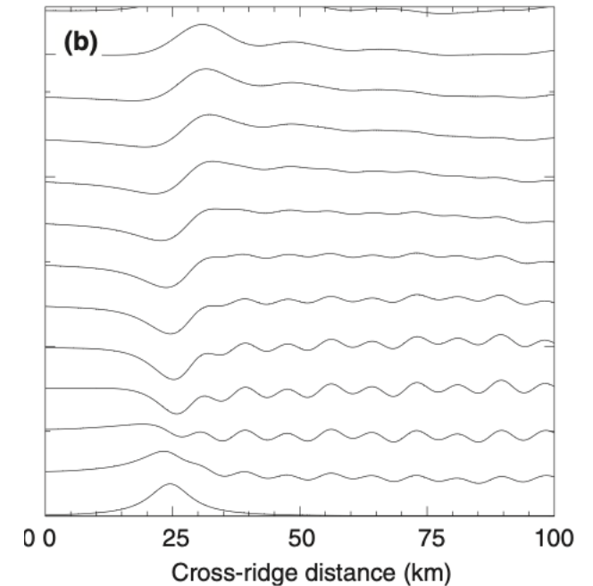
Streamlines in steady air flow over an isolated mountain as predicted by linear theory (Durran, 2015).
