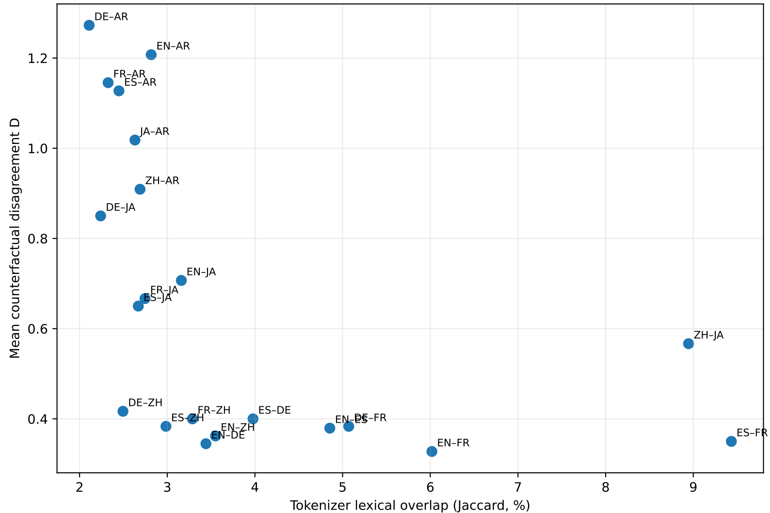
Primary: lexical overlap vs counterfactual disagreement Spearman \rho = -0.782
