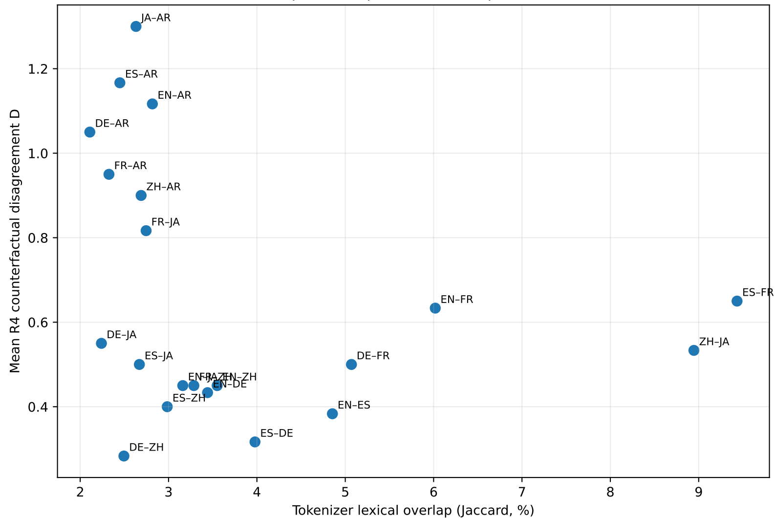
R4: lexical overlap vs disagreement Spearman \rho=-0.401 , QAP \rho=0.12
