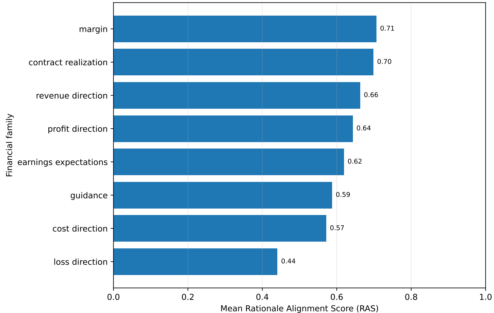
R4 rationale alignment by financial relation type
