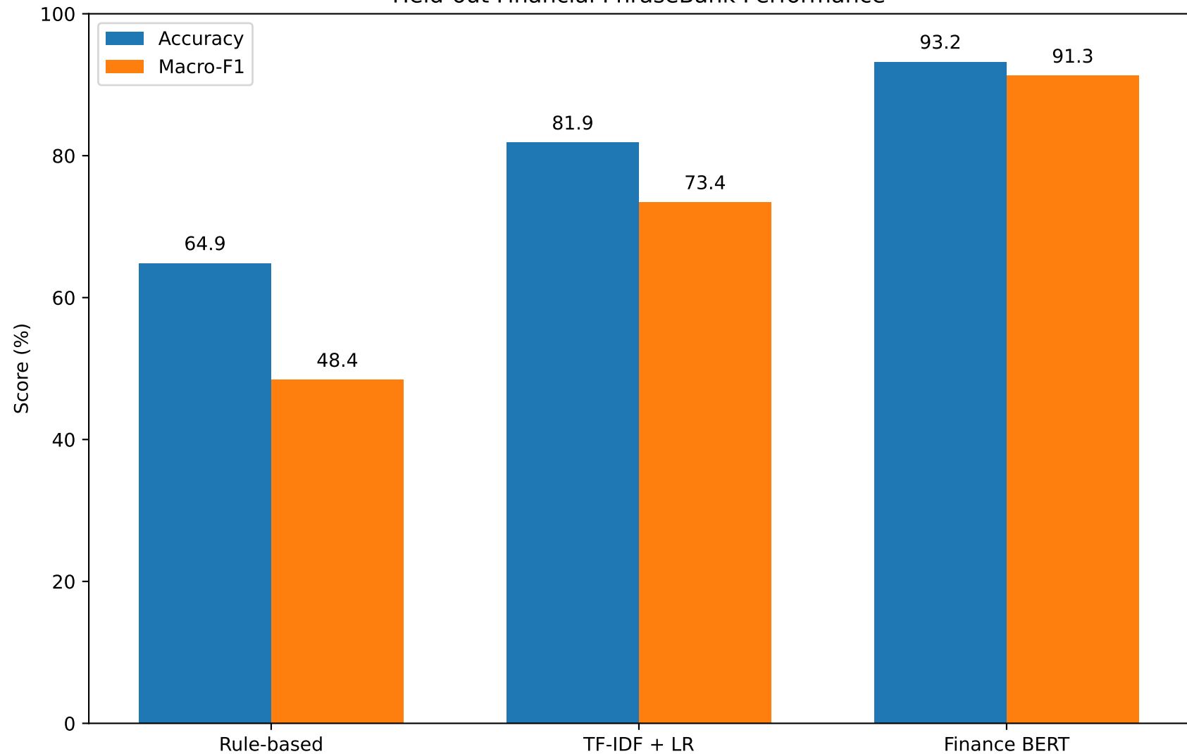
Held-out Financial PhraseBank Performance
