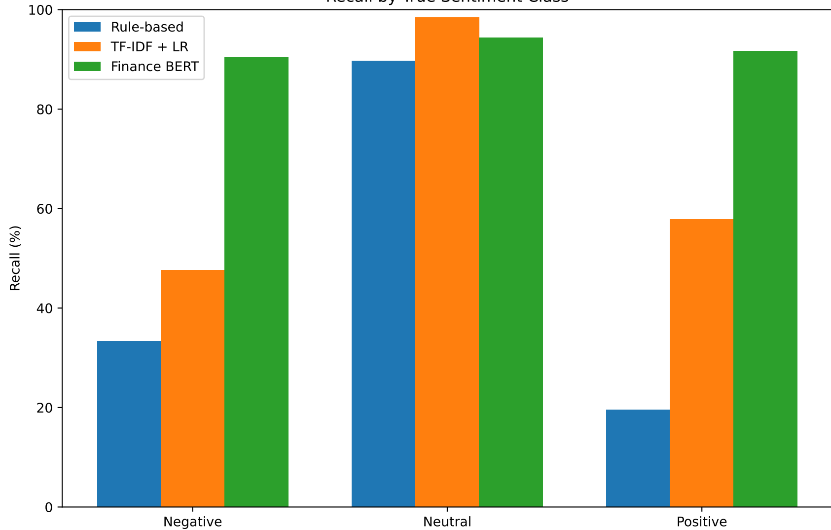
Recall by True Sentiment Class
