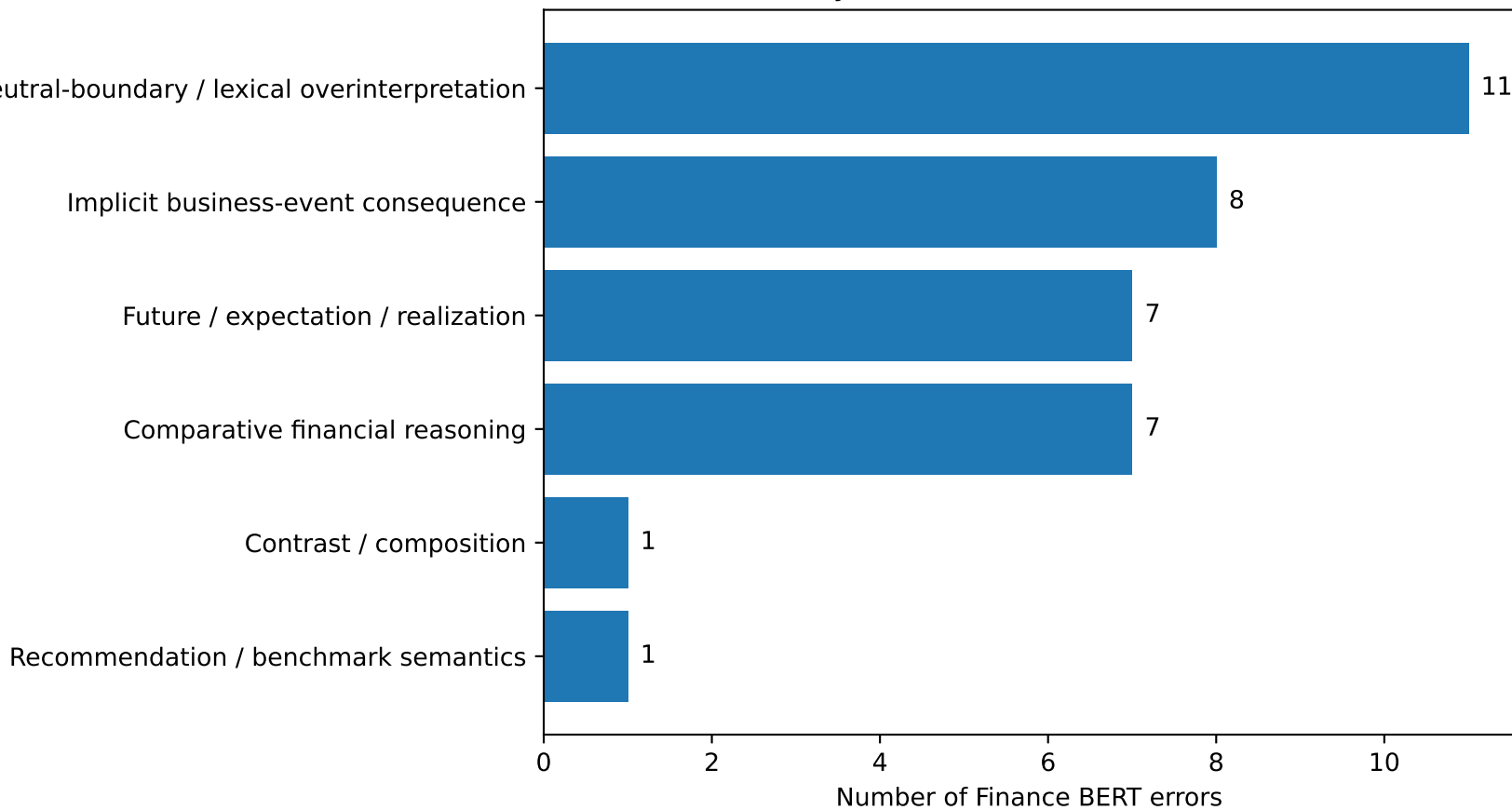
Taxonomy of All 35 Finance BERT Test Errors
