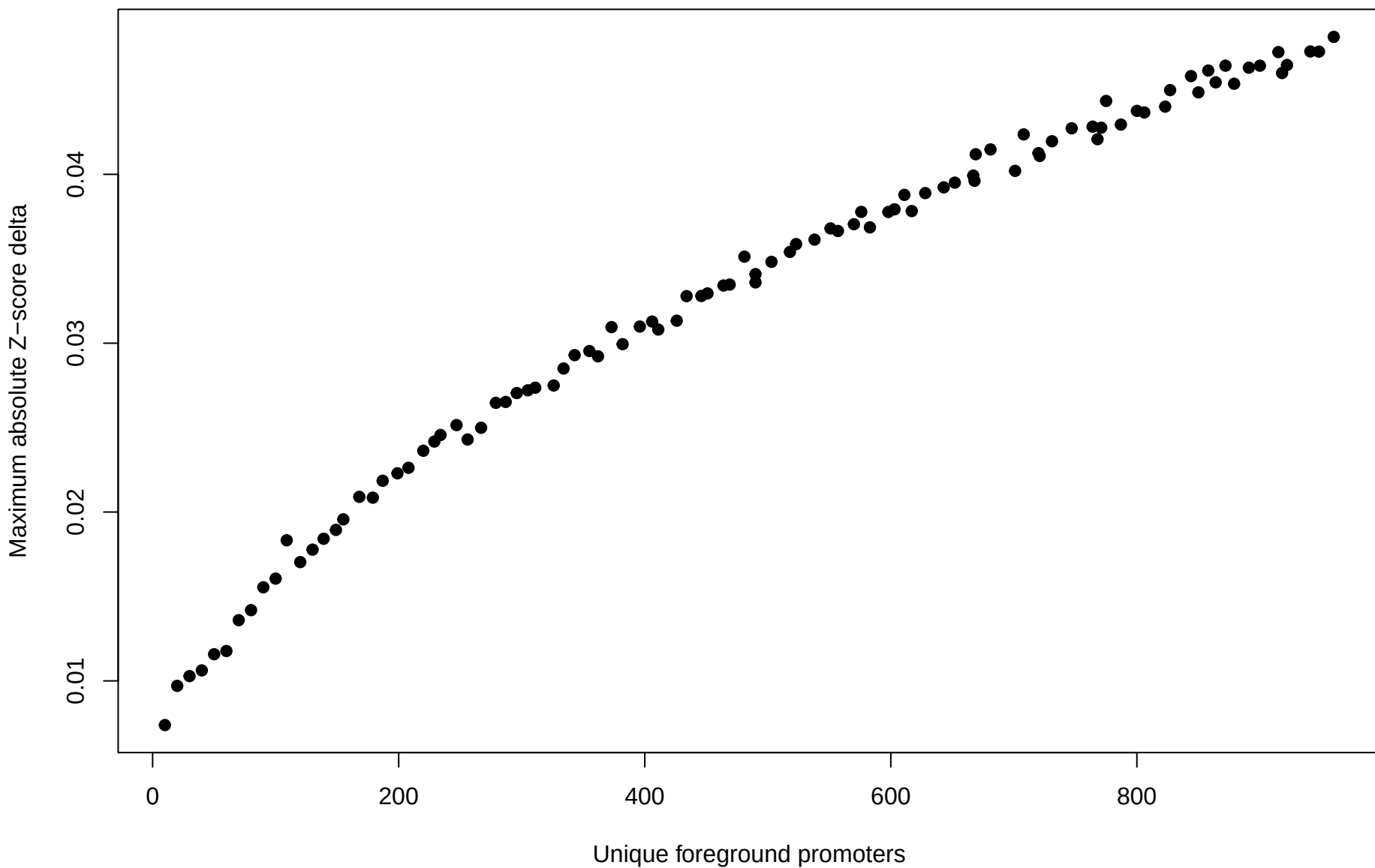
Downstream benchmark Z-score impact
