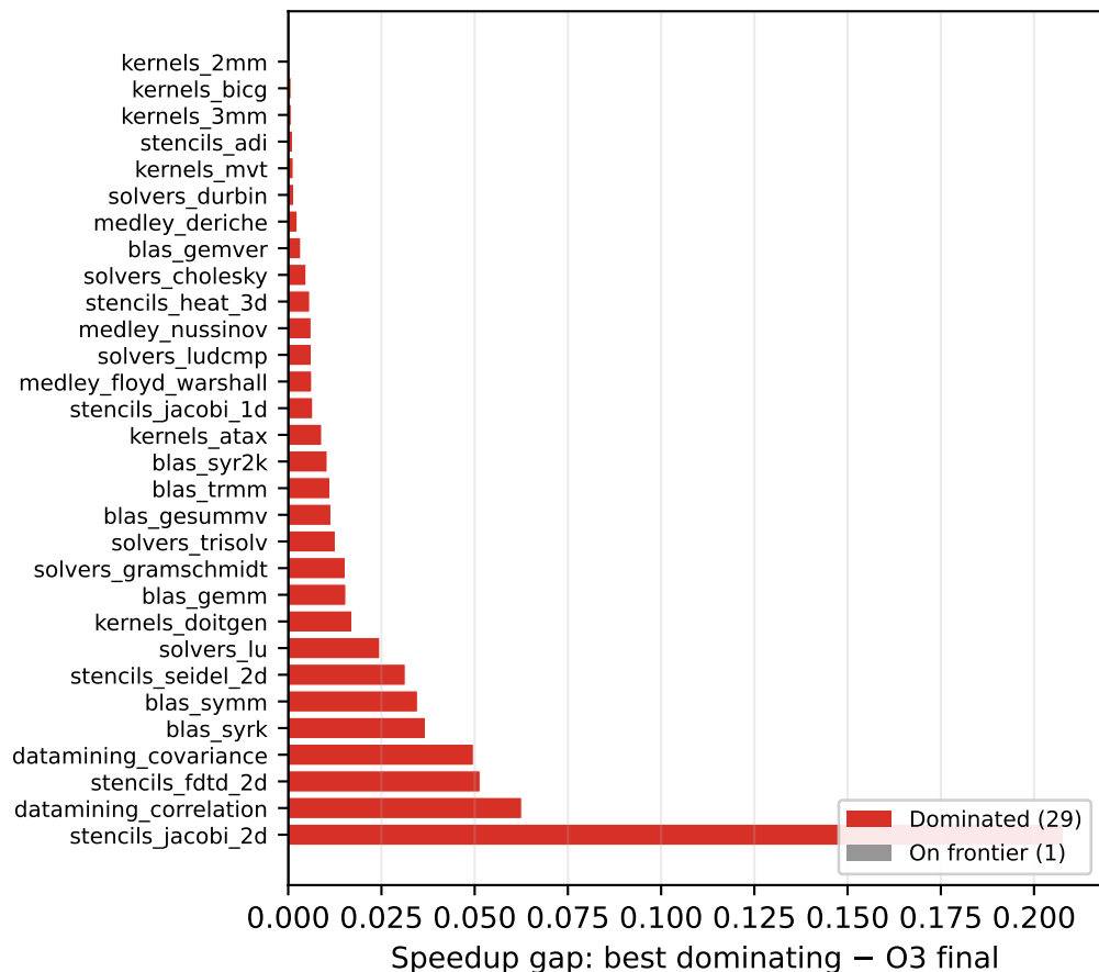
Panel B — Per-benchmark speedup gap (29/30 benchmarks have gap > 0)
