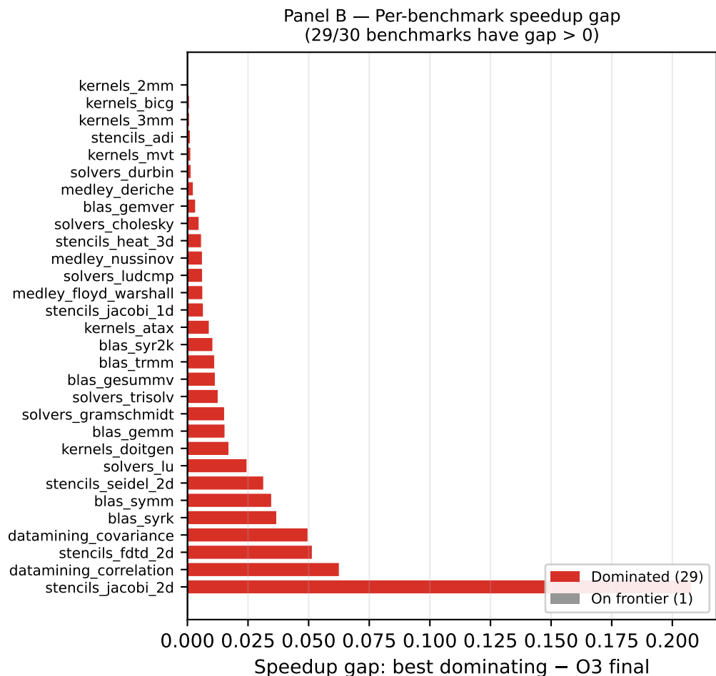
Figure 13e · Pareto Dominance: Final O3 vs. Earlier Checkpoints (Binary Size & Speedup)
