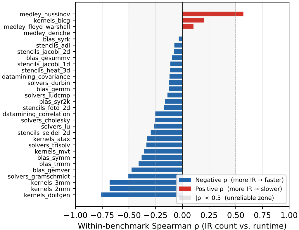
Panel B — Per-benchmark \rho (sorted) 25/30 have |\rho| < 0.5 | mean \rho = -0.22
