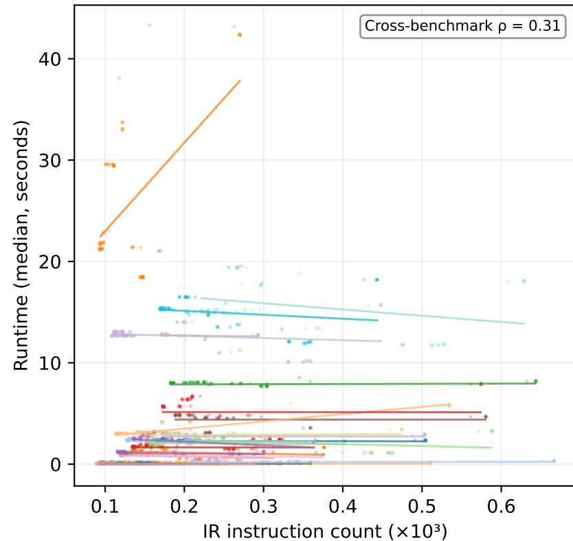
Panel A — IR count vs. runtime (per-benchmark regression lines)
