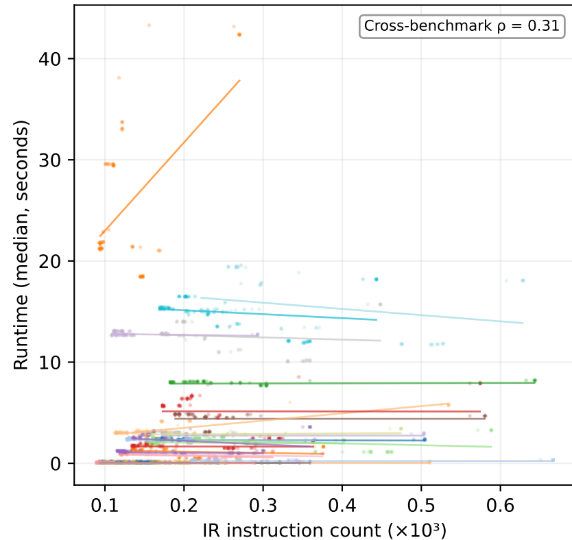
Panel A — IR count vs. runtime (within-benchmark regression lines)
