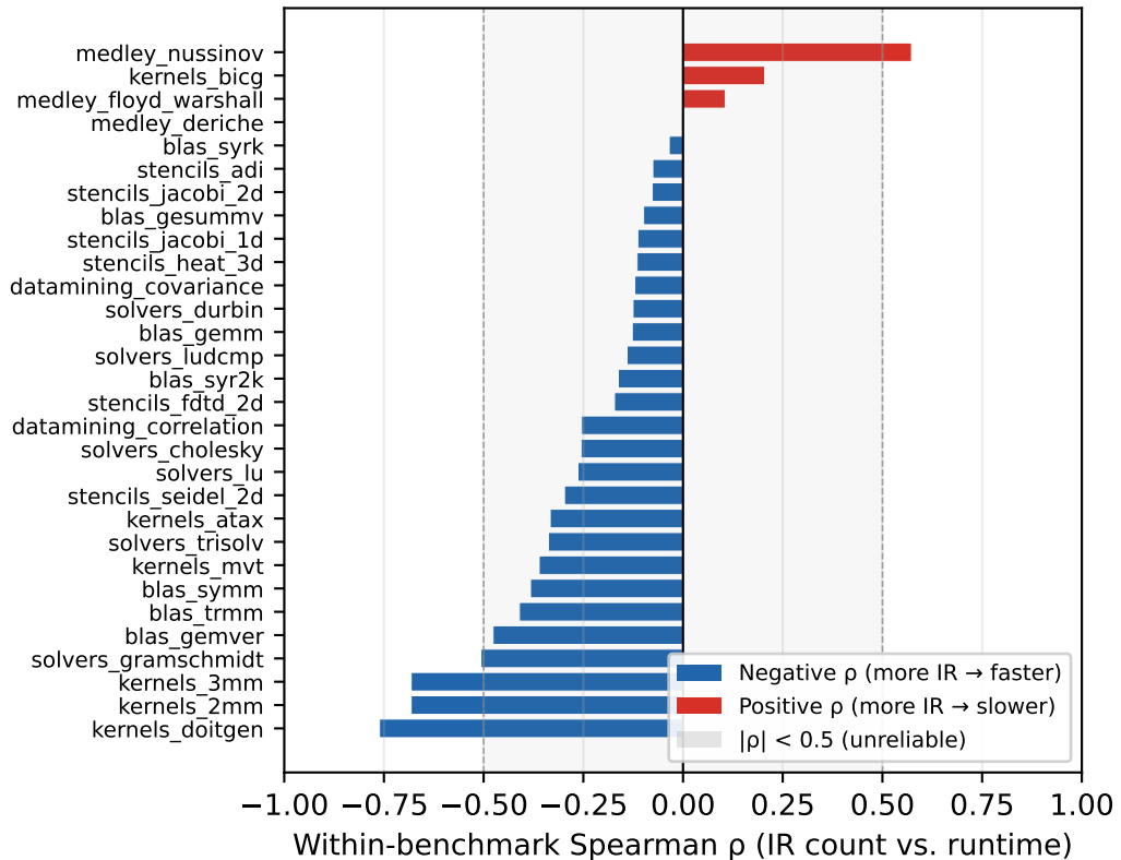
Panel B — Per-benchmark Spearman \rho (25/30 benchmarks have |\rho| < 0.5 )
