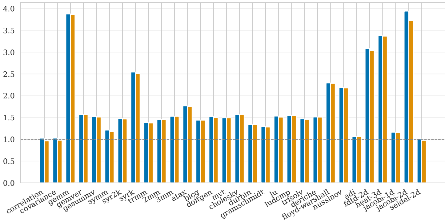
Speedup vs O0 (Median)
