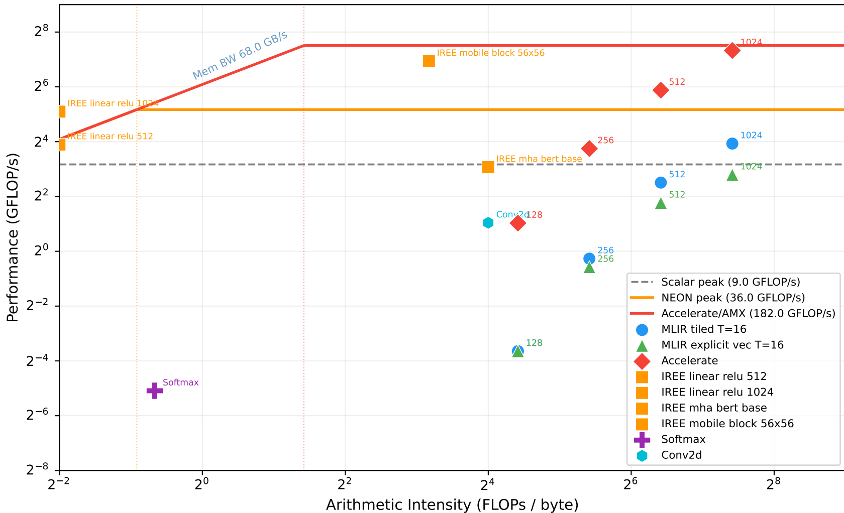
Roofline — Apple M4 Pro (single thread, FP32) MLIR tiled T=16 · MLIR explicit vec · IREE · Accelerate/AMX
