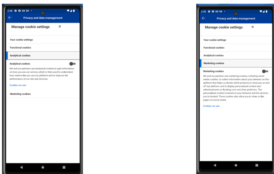
Figure 4: Booking.com privacy settings screen showing analytics and marketing tracking disabled after appInterface.postMessage("dnsmi") invocation.
