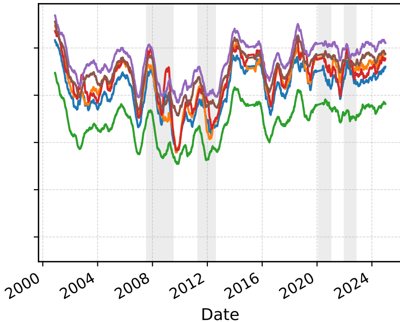
Rolling 6-Month Turnover by Quintile (Muon Optimizer)
