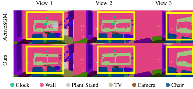
Fig. 2. Novel-view semantic rendering comparison in Replica. The yellow boxes highlight a screen region where ActiveSGM changes labels across views, while ActiveSIGMA retains a more stable label.
