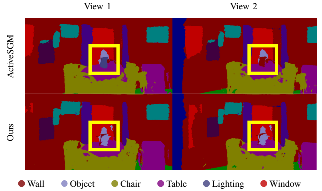
Fig. 3. Novel-view semantic rendering comparison in MP3D. The yellow boxes highlight a table-top vase whose label changes across views with ActiveSGM but remains stable with ActiveSIGMA.
