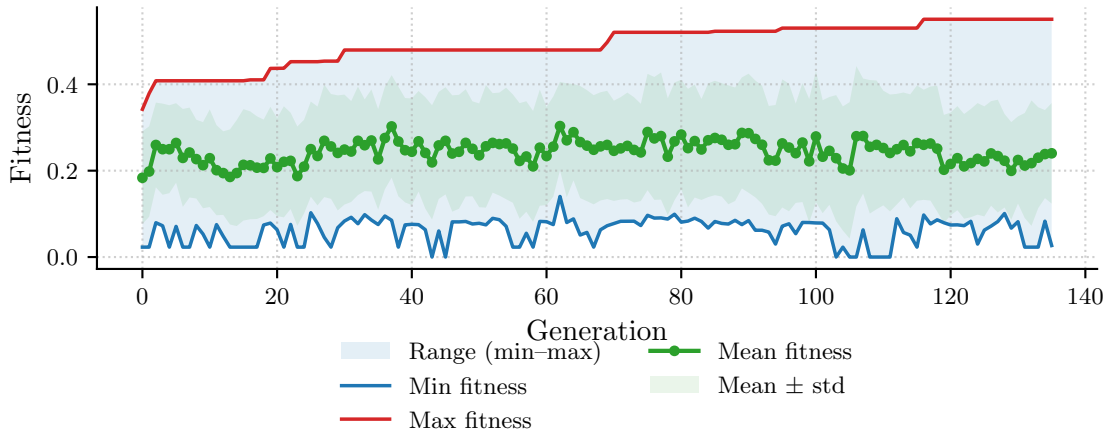
Evolution of fitness over generations
