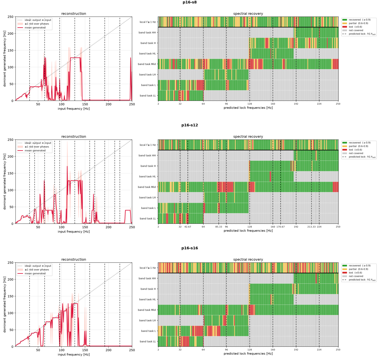
Figure 1: The three P=16 geometries under a pure-sinusoid sweep at 1 Hz. The stride lengthens from S=8 at the top to S=16 at the bottom while the patch grid stays fixed, so a feature that moves between rows belongs to the stride branch. Left: generated against given frequency, a point on the diagonal being a tone rebuilt correctly. Right: whether that frequency is still recoverable from the representation, one row per probing task; green recovered, red lost, grey not covered. Dashed lines mark F_{lock} .
