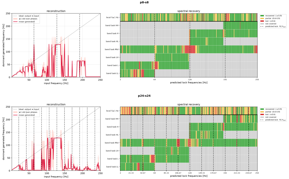
Figure 2: The two geometries with P=S , drawn and read as in Figure 1. Here the two branches coincide, so one set of dashed lines covers both and neither geometry can attribute a dip to one of them. They vary the patch length at zero overlap, which anchors the patch-size axis of the configuration-level regression.
