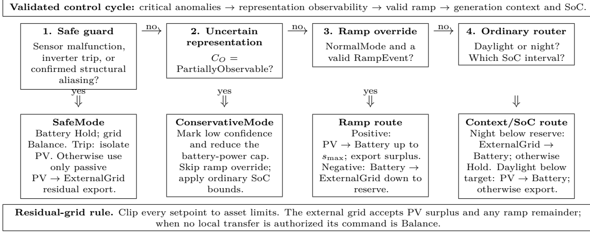
Figure 1: Routing-policy flowchart. Gates are evaluated from left to right according to the strict precedence in Eq. (15).
