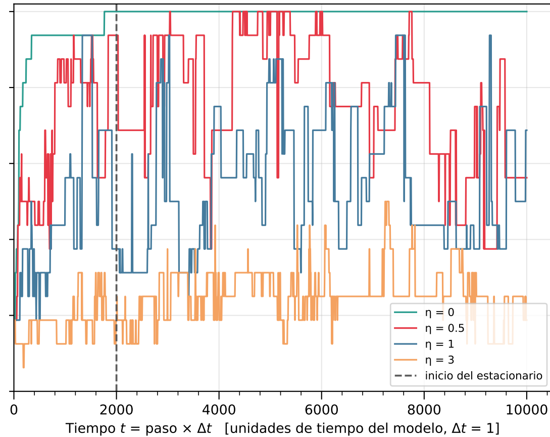
\rho = 0.16 ( N = 16, L = 10 )
