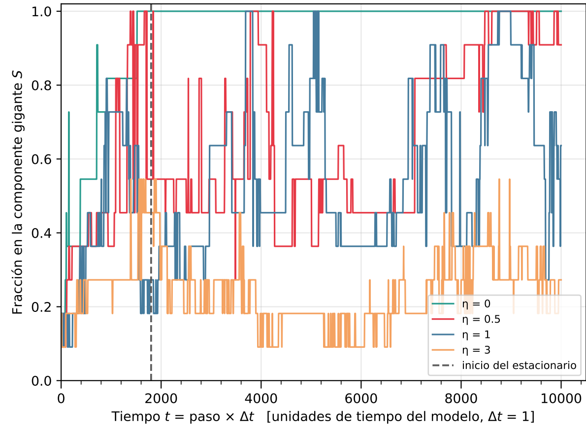
\rho = 0.11 ( N = 11, L = 10 )
