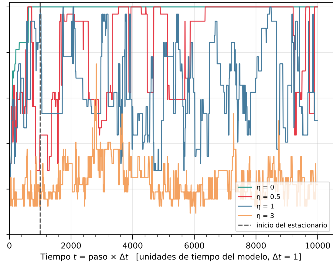
\rho = 0.32 ( N = 32, L = 10 )
