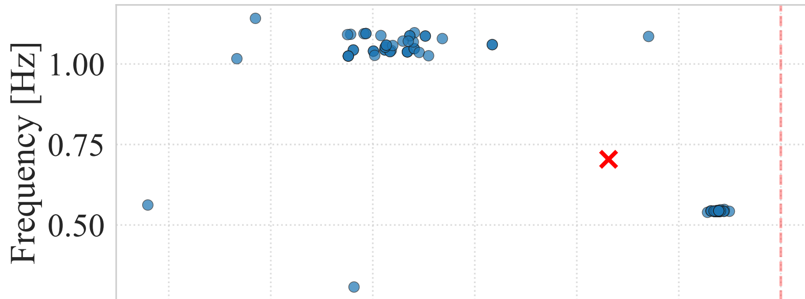
k – Means Results: k = 1 WCSS: 286.0
