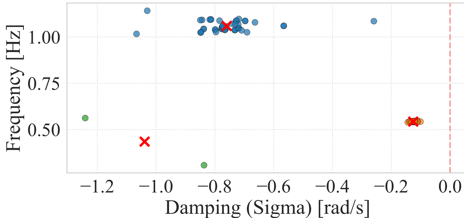
k – Means Results: k = 3 WCSS: 8.0
