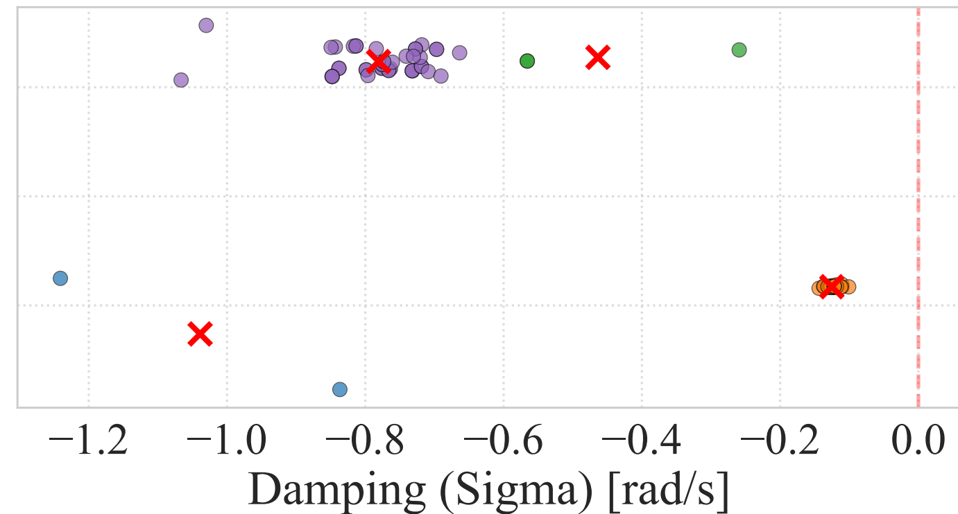
k – Means Results: k = 4 WCSS: 5.2
