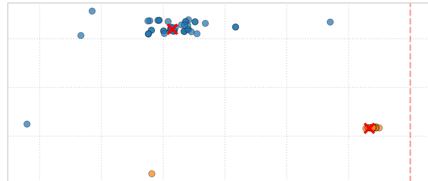
k – Means Results: k = 2 WCSS: 19.2
