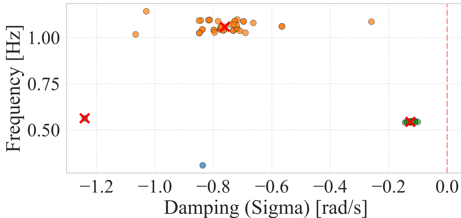
k – Medoids Results: k = 3 Cost: 14.1
