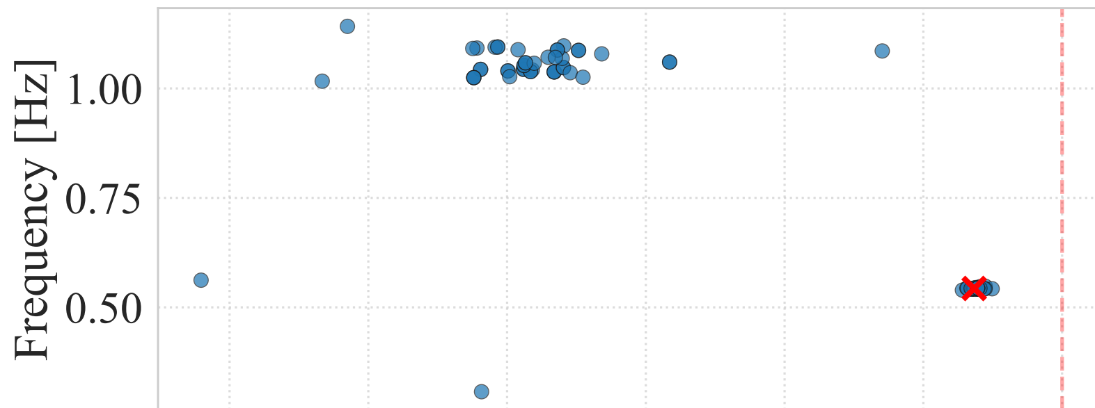
k – Medoids Results: k = 1 Cost: 140.0
