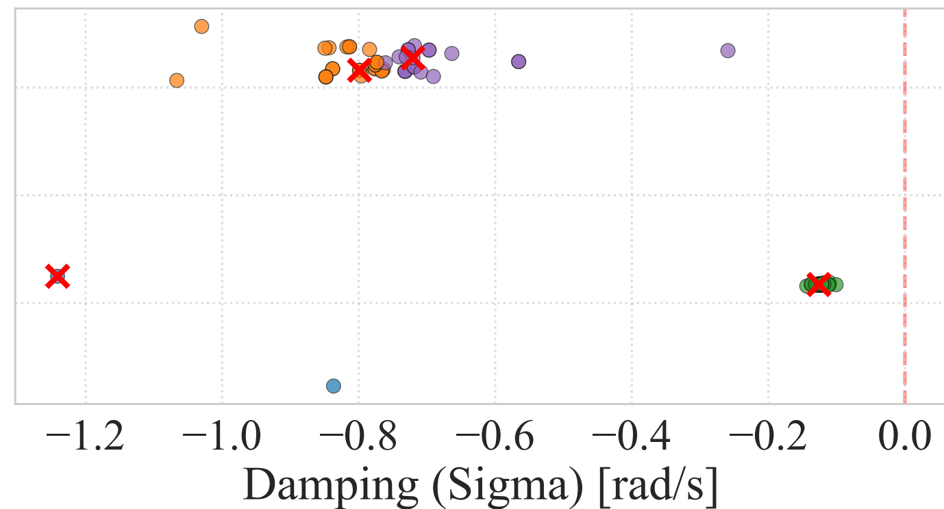
k – Medoids Results: k = 4 Cost: 11.8
