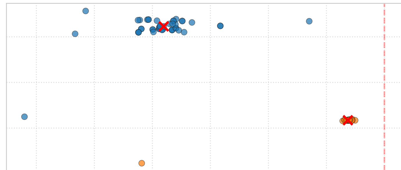
k – Medoids Results: k = 2 Cost: 17.4
