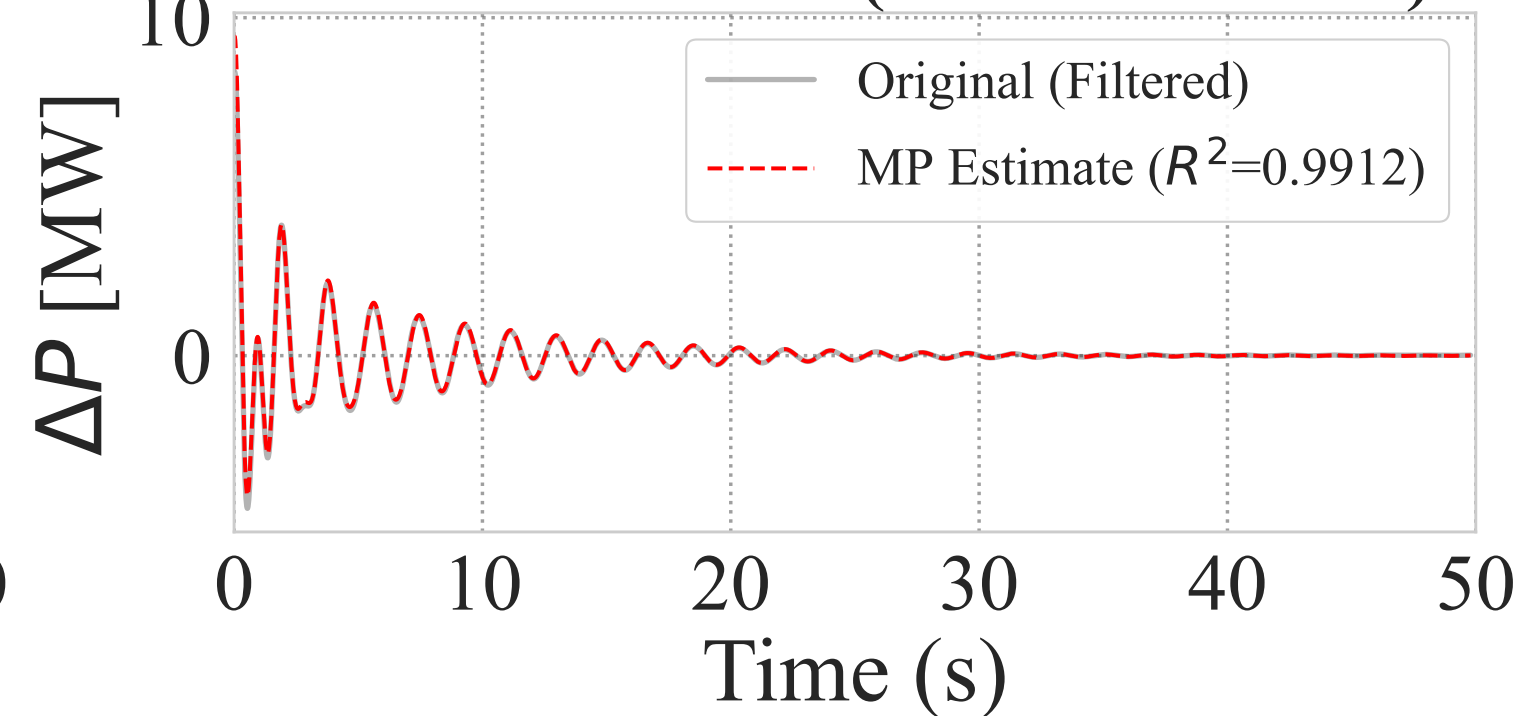
Method: Tau 0.01 (RMSE: 7.82e-02)
