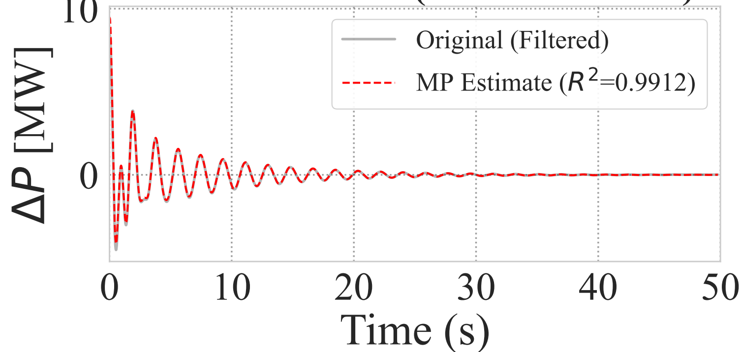
Method: Order 6 (RMSE: 7.82e-02)
