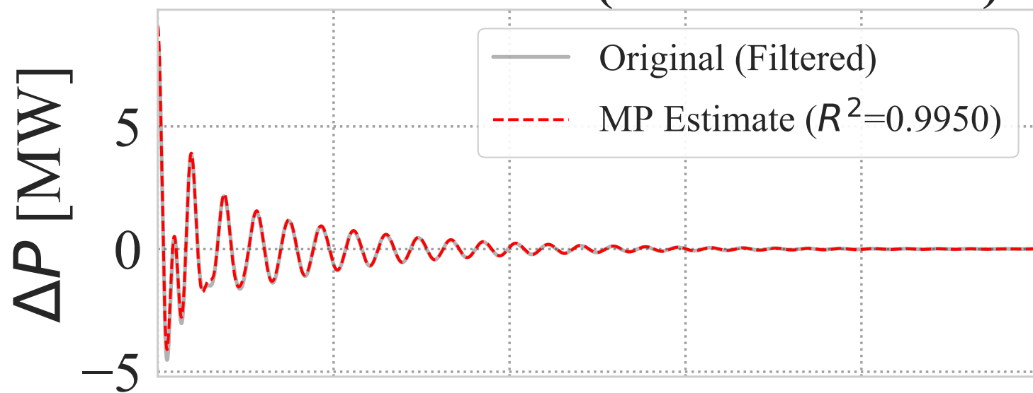
Method: Order 4 (RMSE: 5.86e-02)
