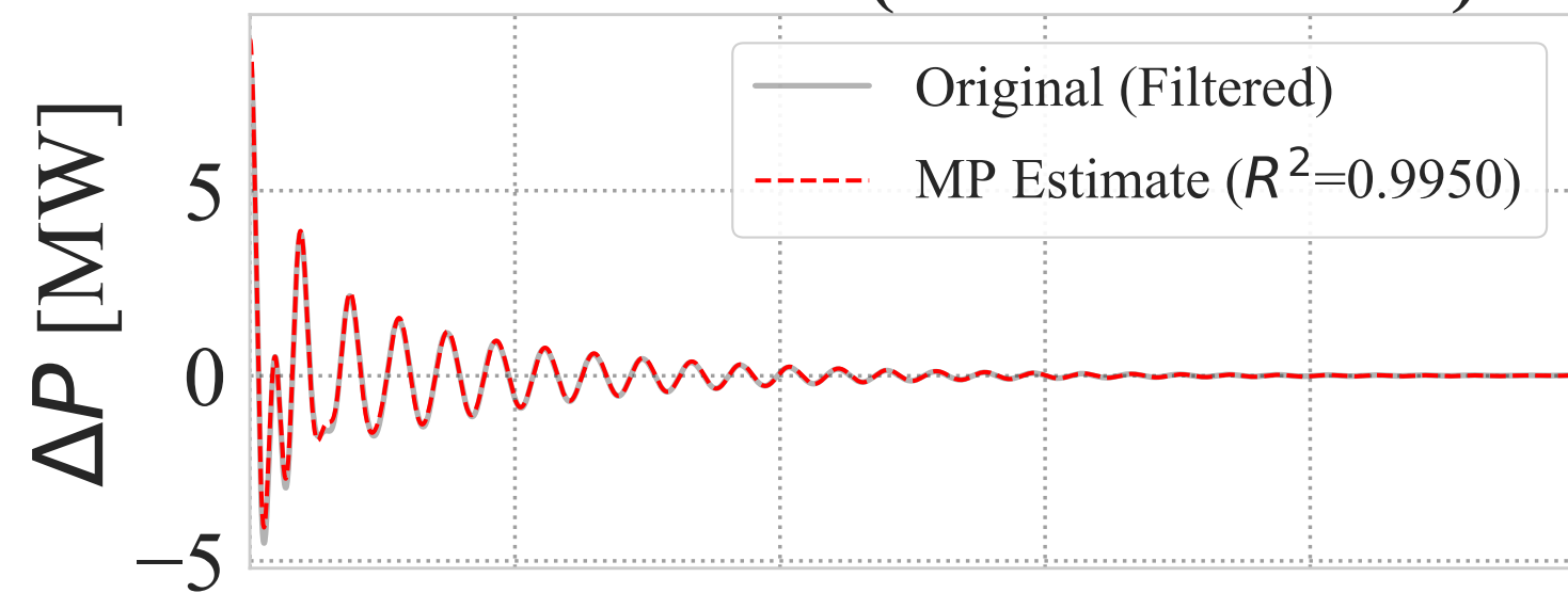
Method: Tau 1 (RMSE: 5.86e-02)
