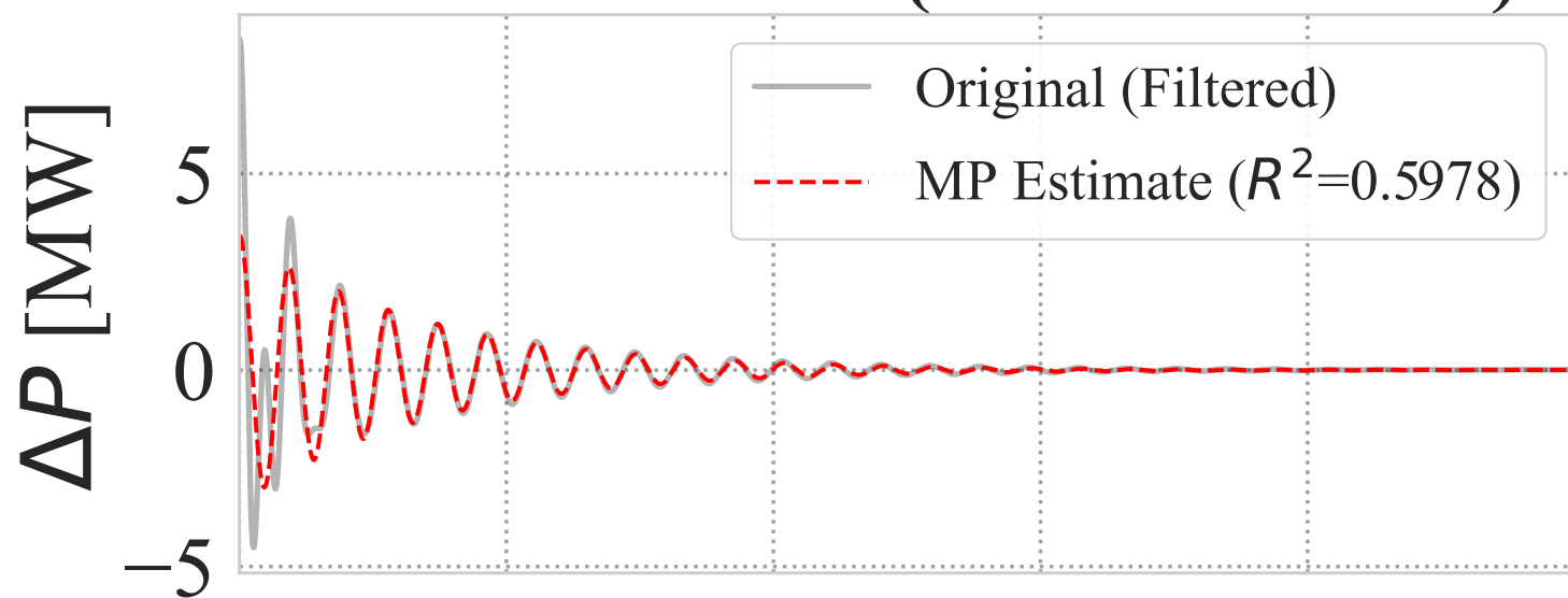
Method: Order 2 (RMSE: 5.28e-01)
