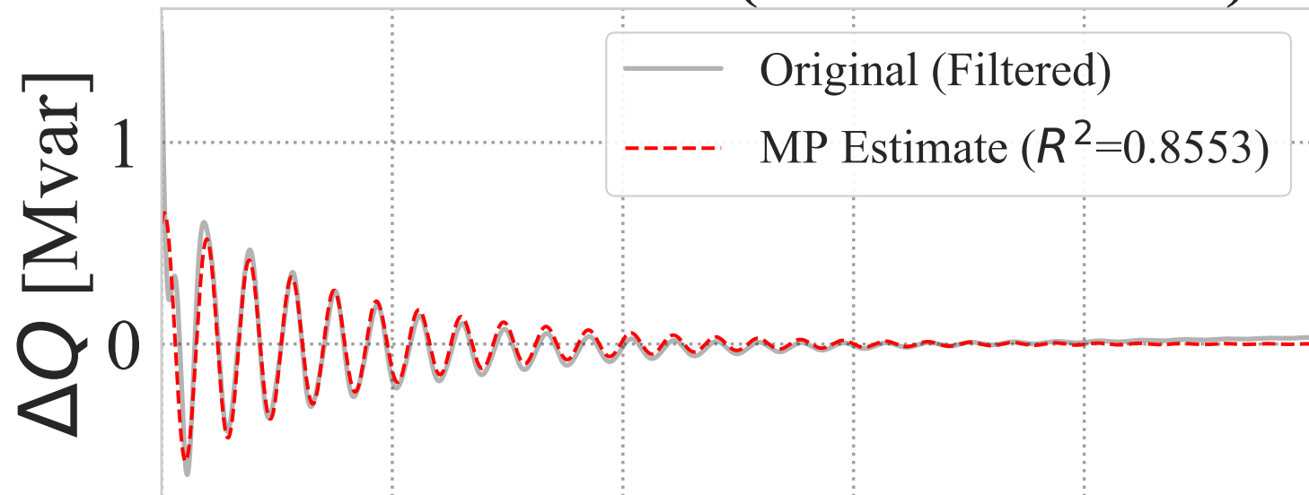
Method: Order 2 (RMSE: 5.61e-02)
