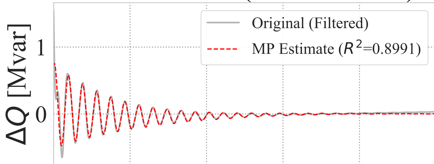
Method: Order 4 (RMSE: 4.68e-02)
