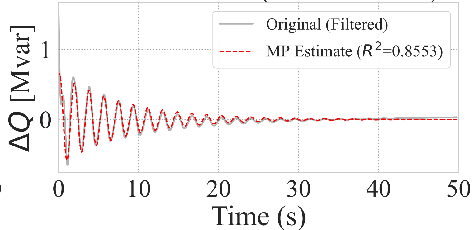
Method: Tau 0.01 (RMSE: 5.61e-02)
