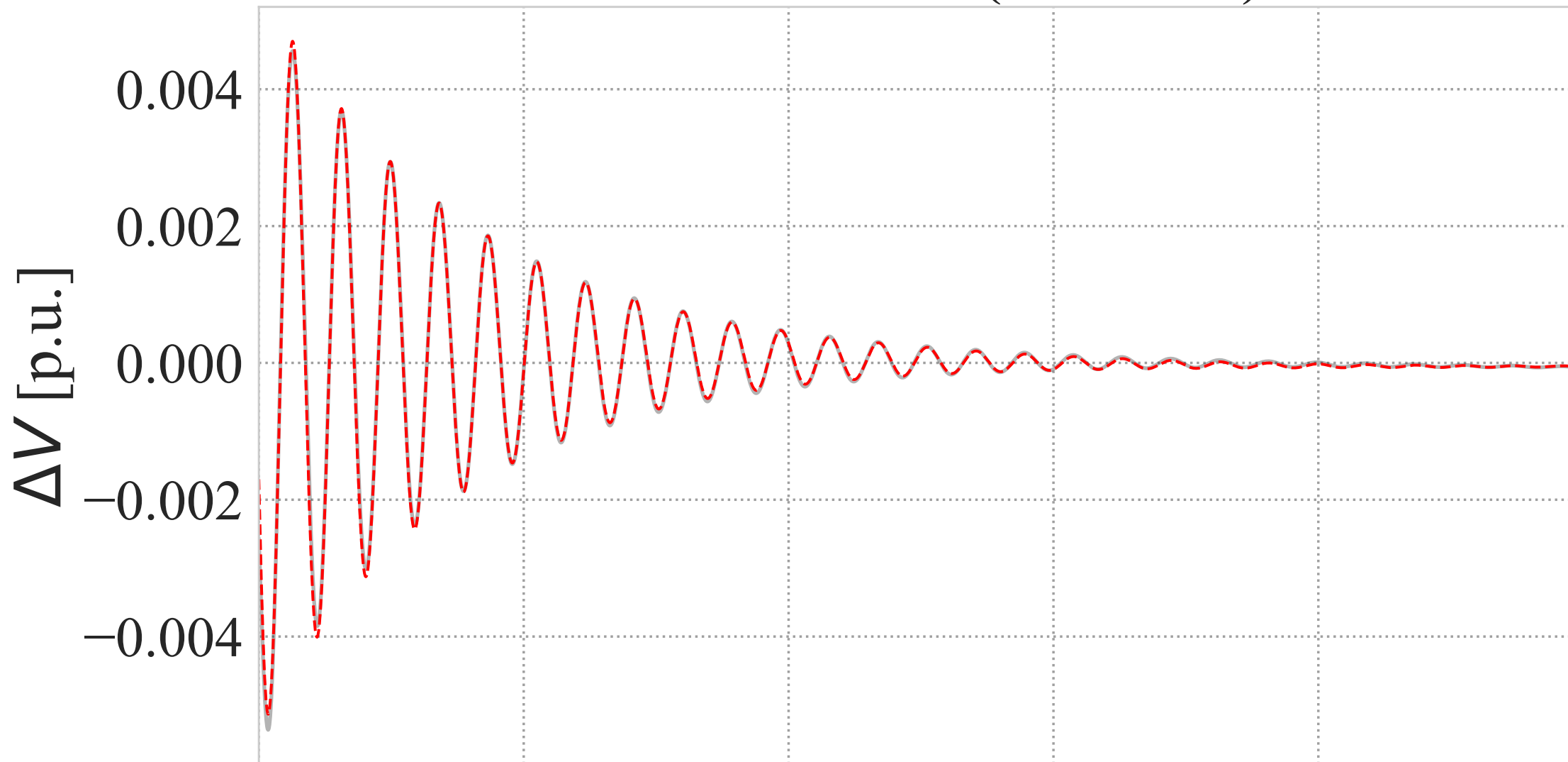
Generator 1 - Voltage
