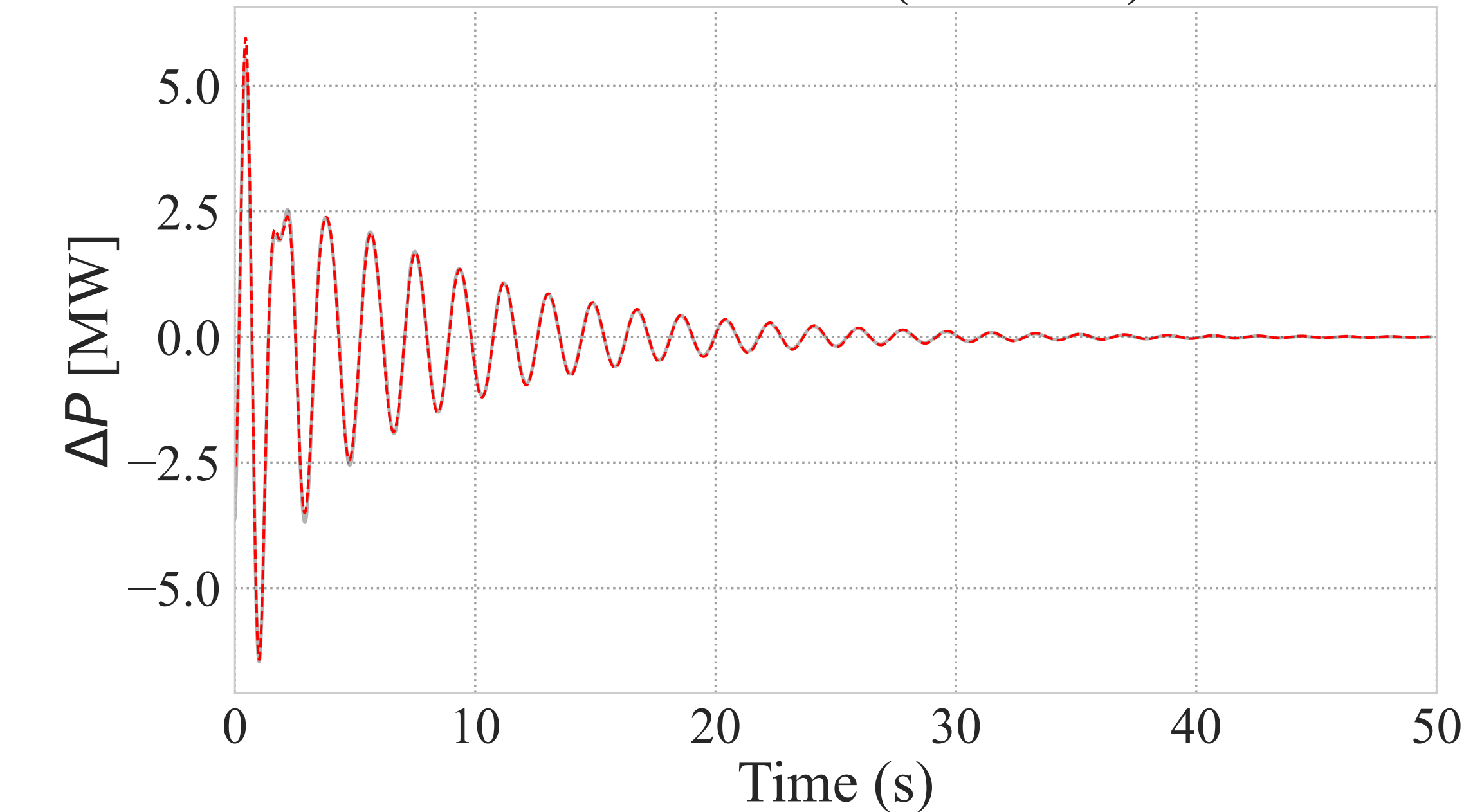
Generator 1 - Active Power
