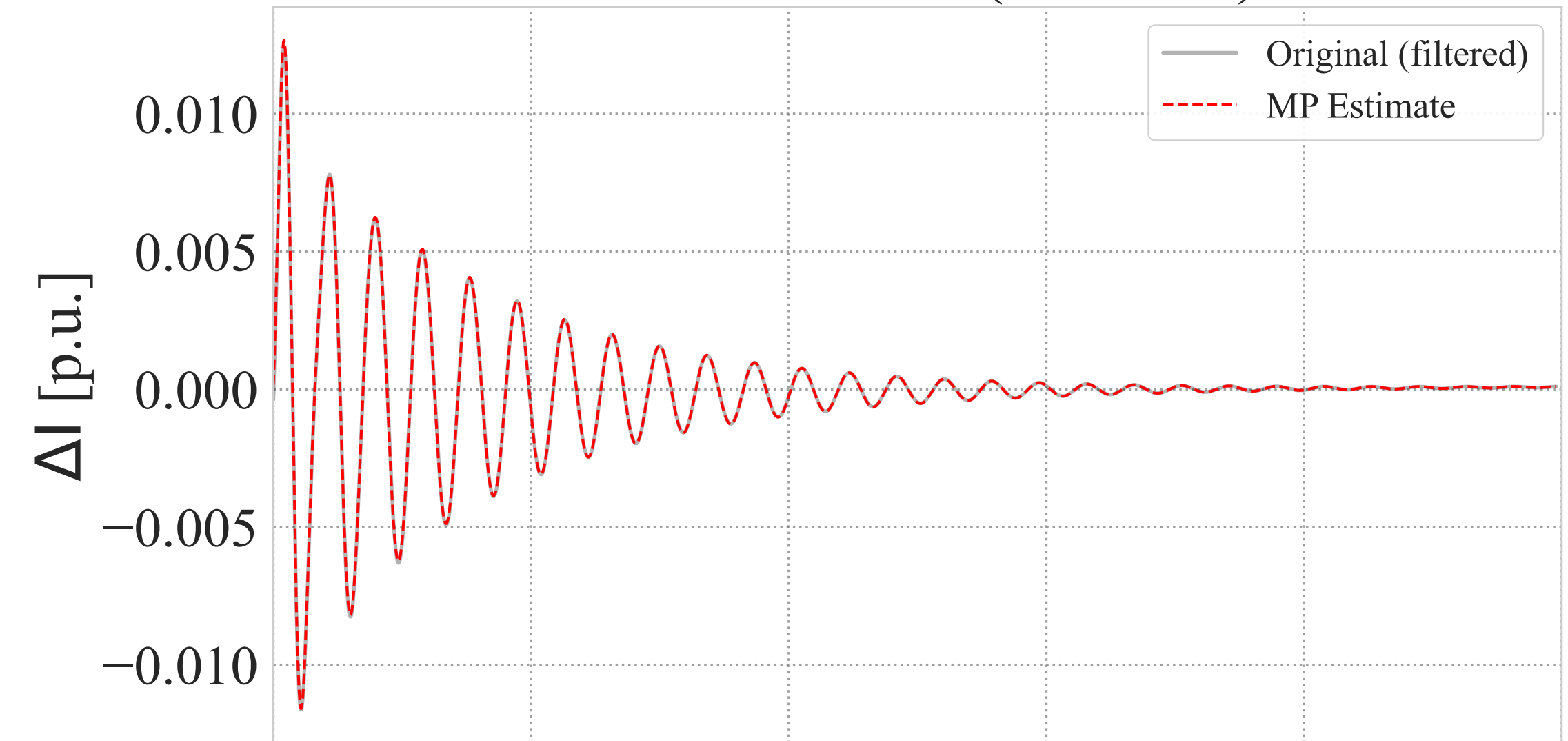
Generator 1 - Current
