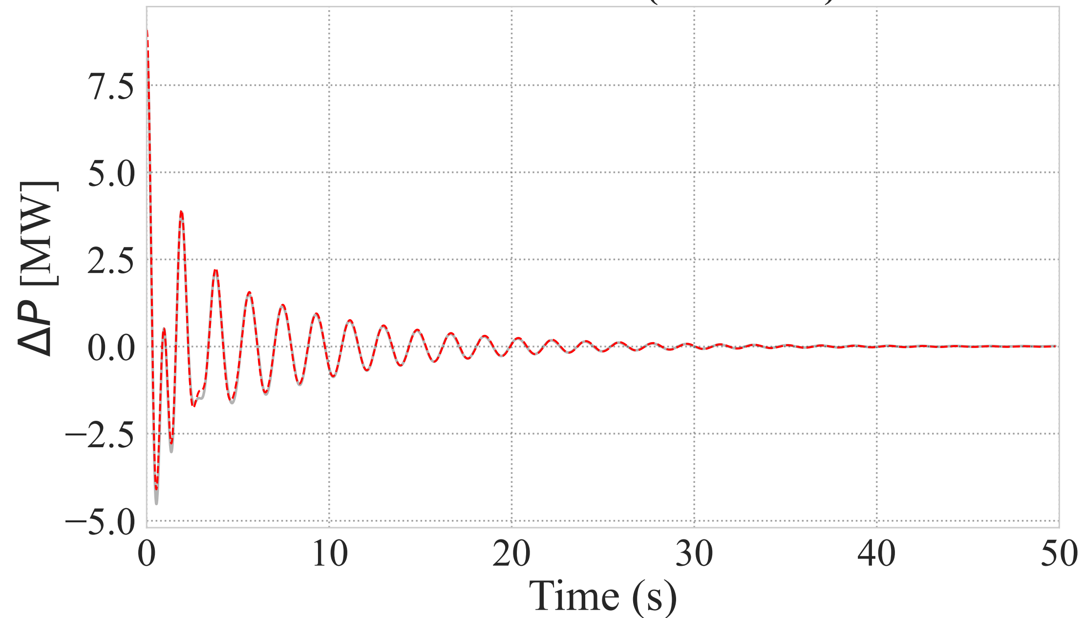
Generator 2 - Active Power
