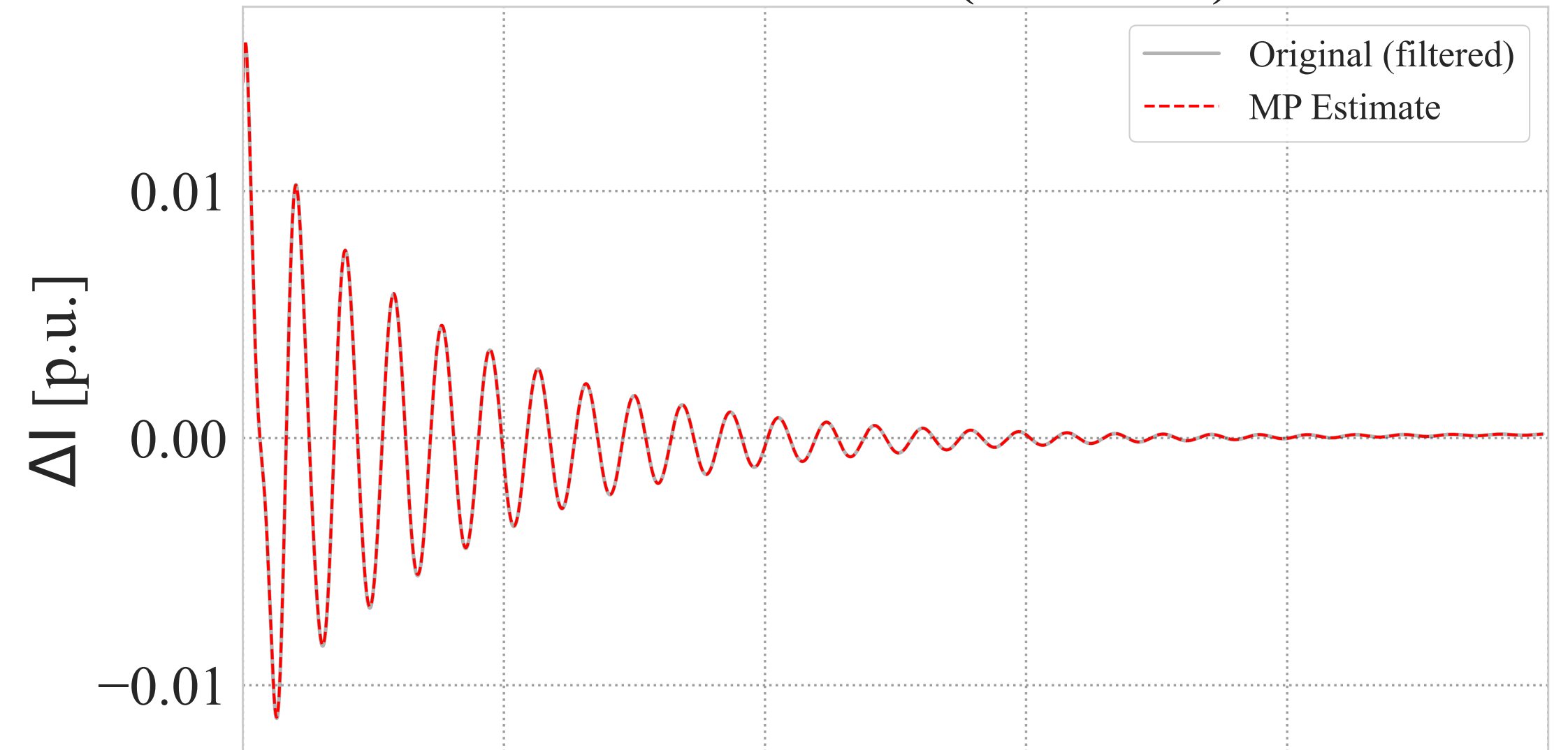
Generator 2 - Current
