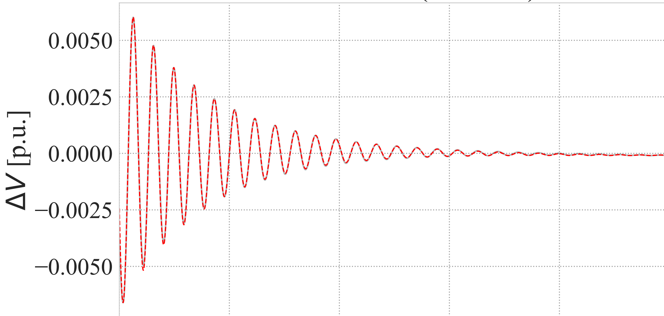
Generator 2 - Voltage
