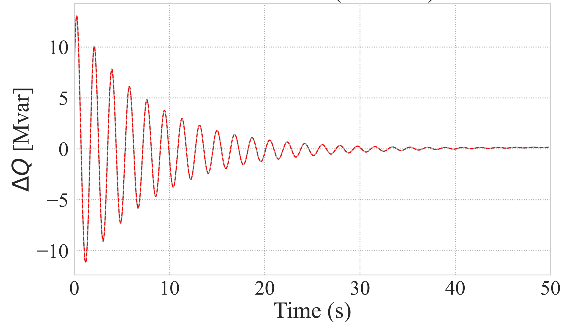
Generator 2 - Reactive Power
