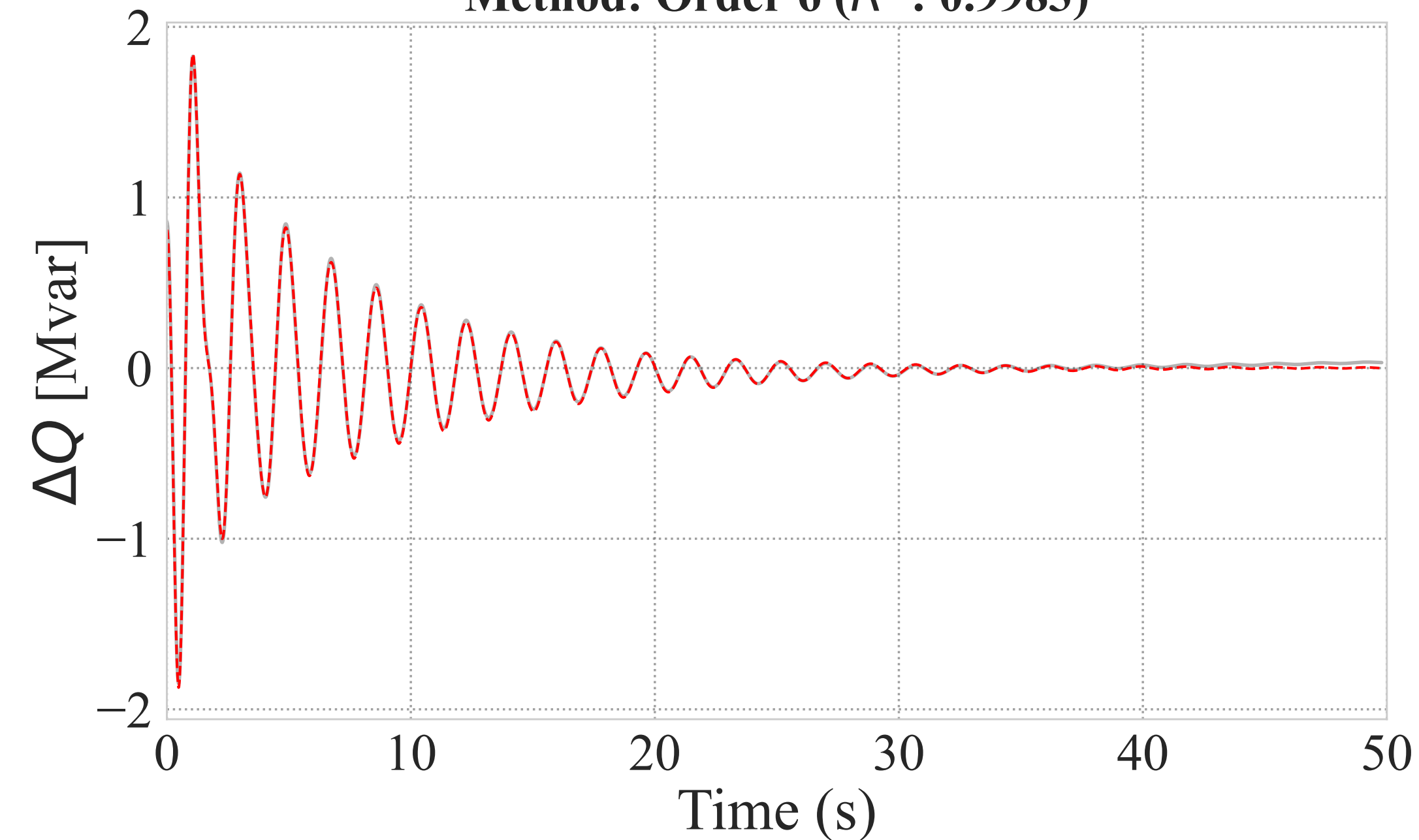
Generator 3 - Reactive Power
