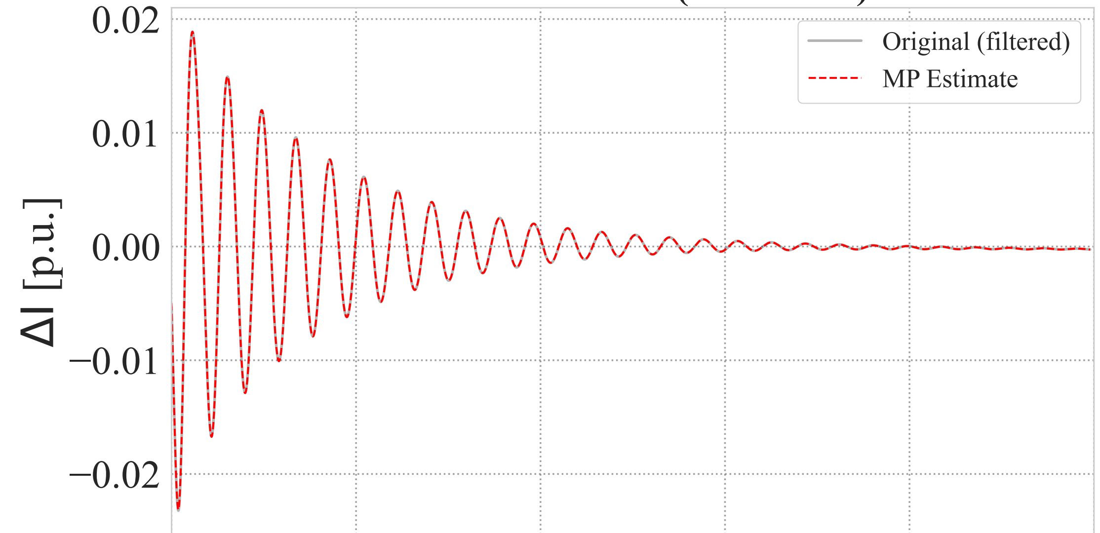
Generator 3 - Current
