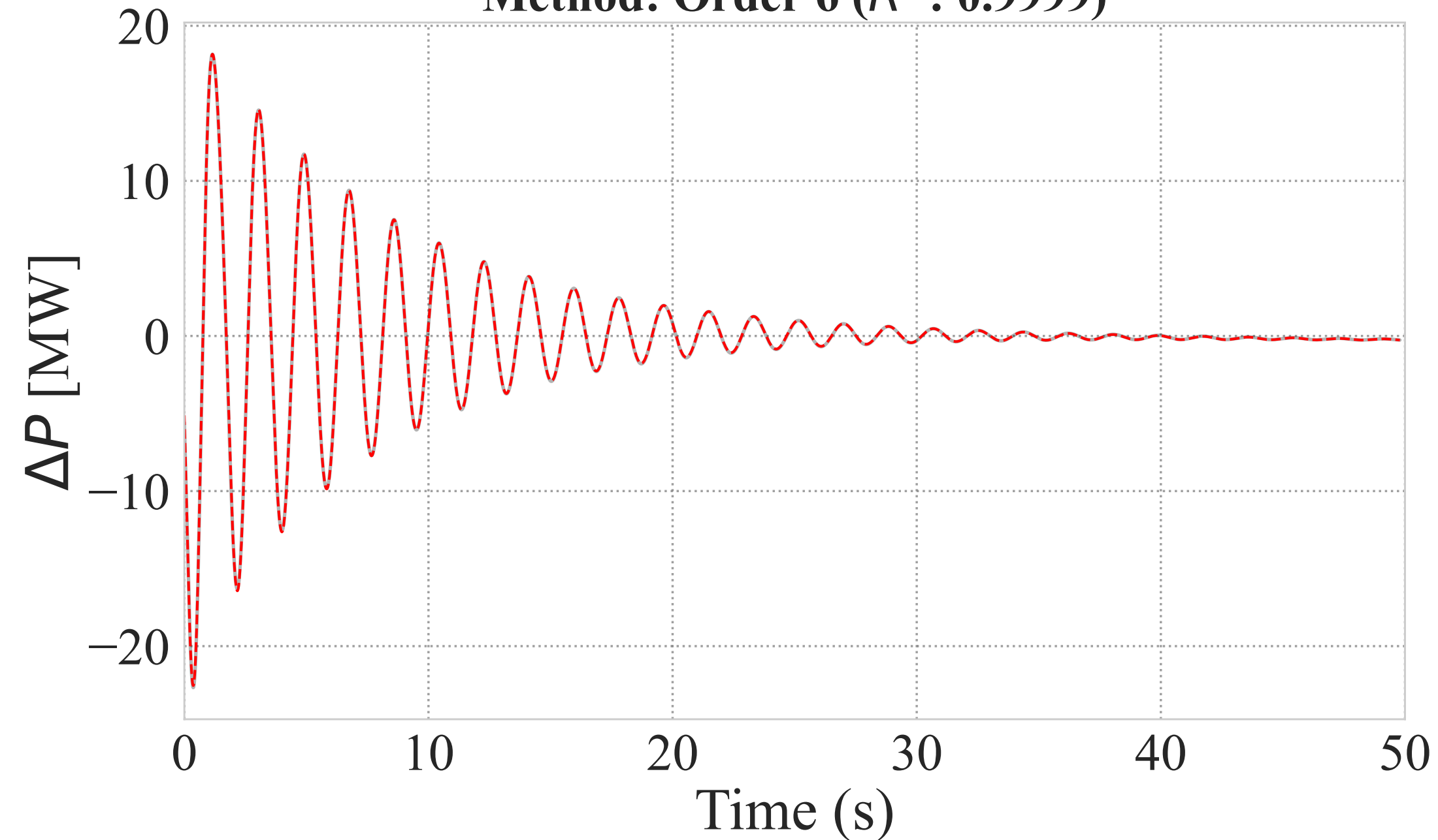
Generator 3 - Active Power
