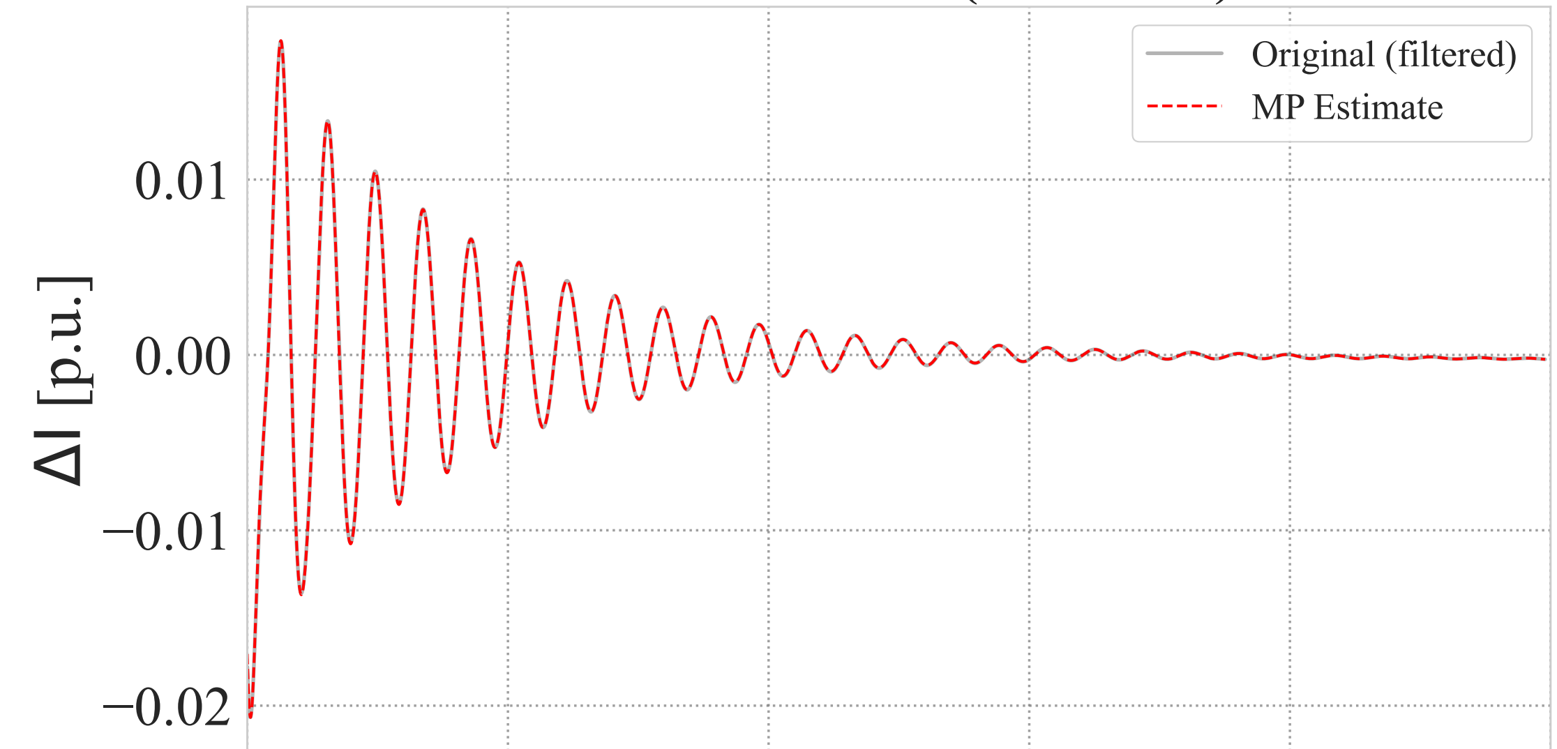
Generator 4 - Current
