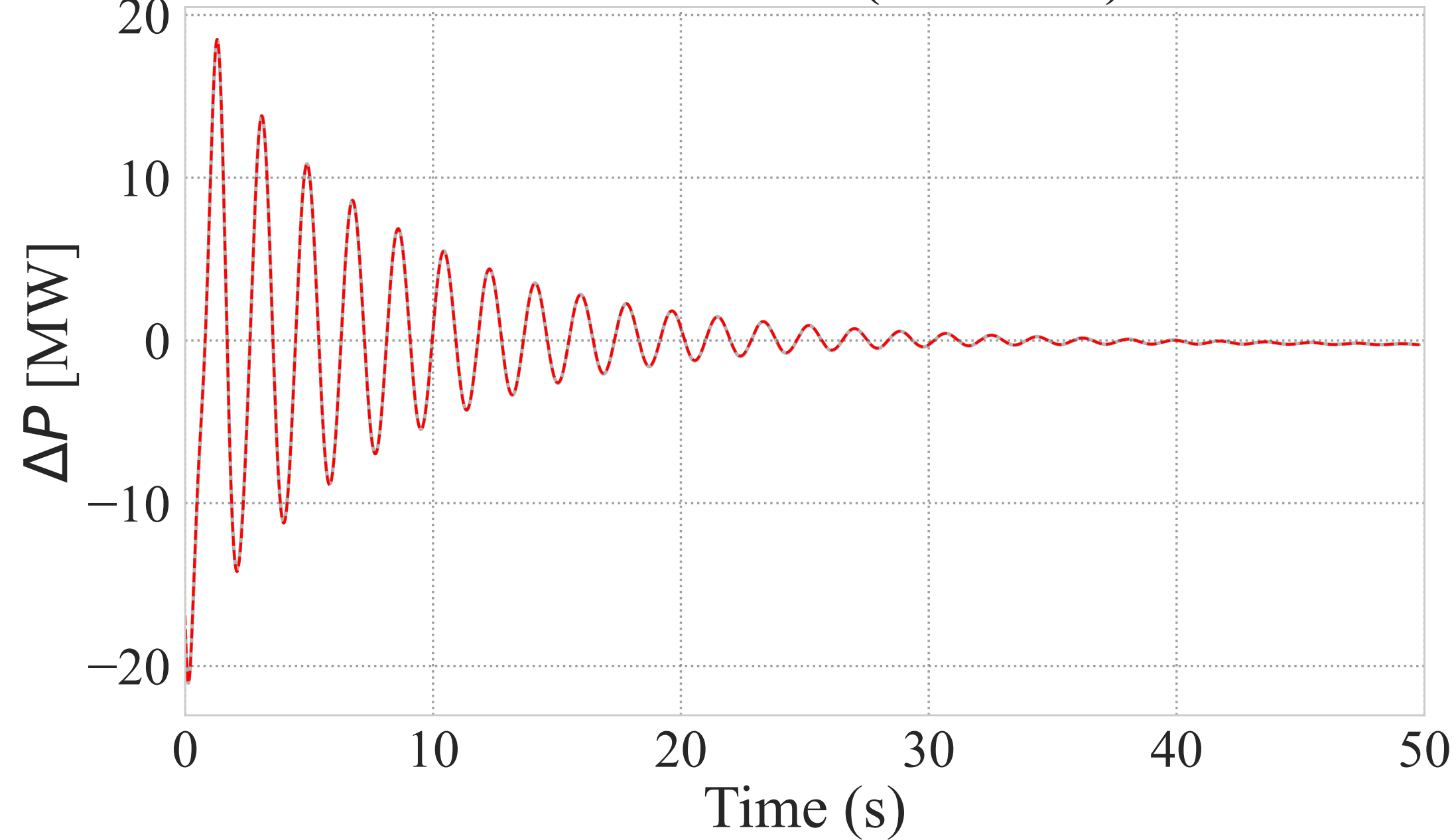
Generator 4 - Active Power
