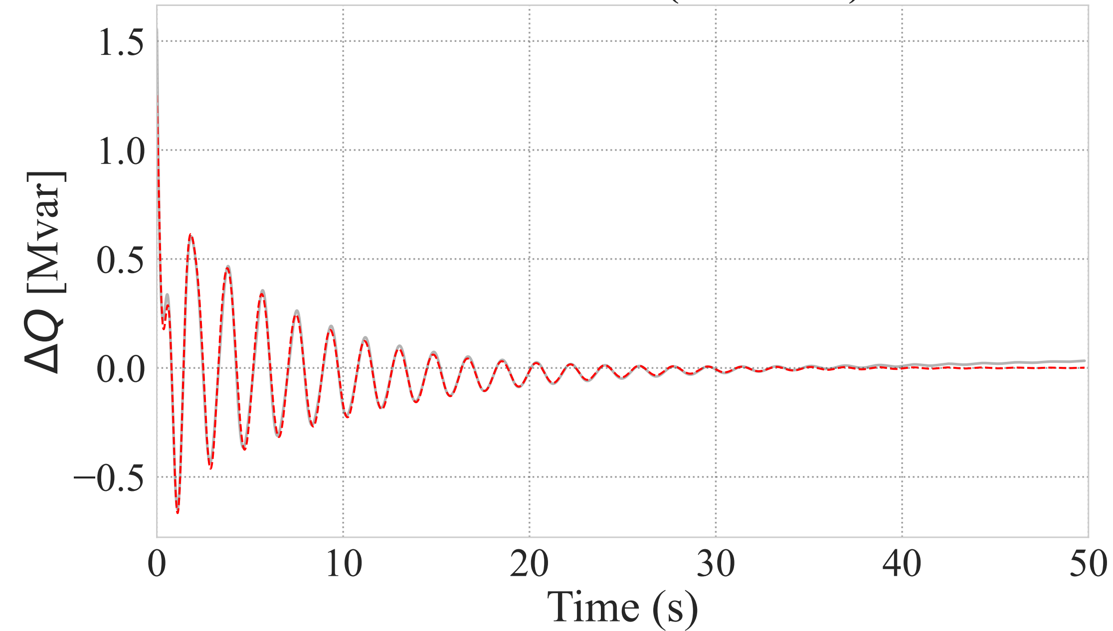
Generator 4 - Reactive Power
