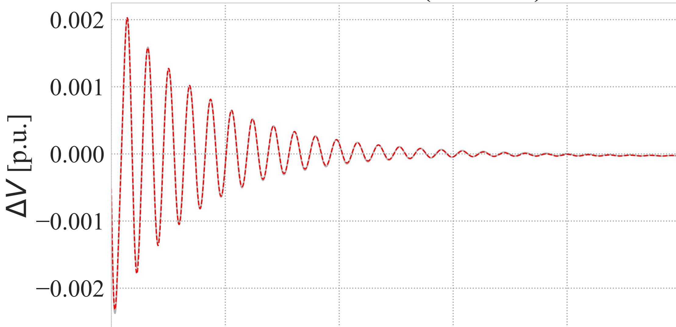
Generator 4 - Voltage
