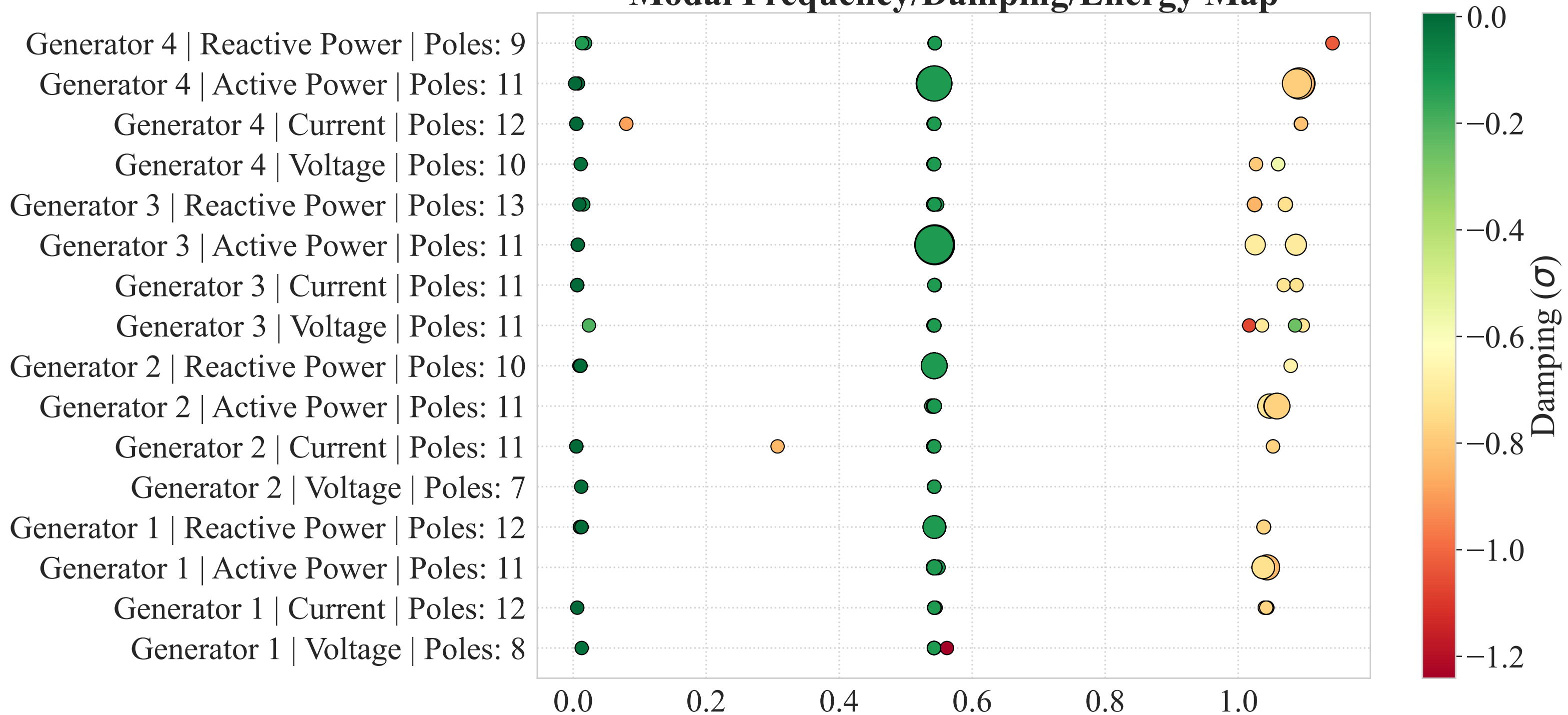
Modal Frequency/Damping/Energy Map
