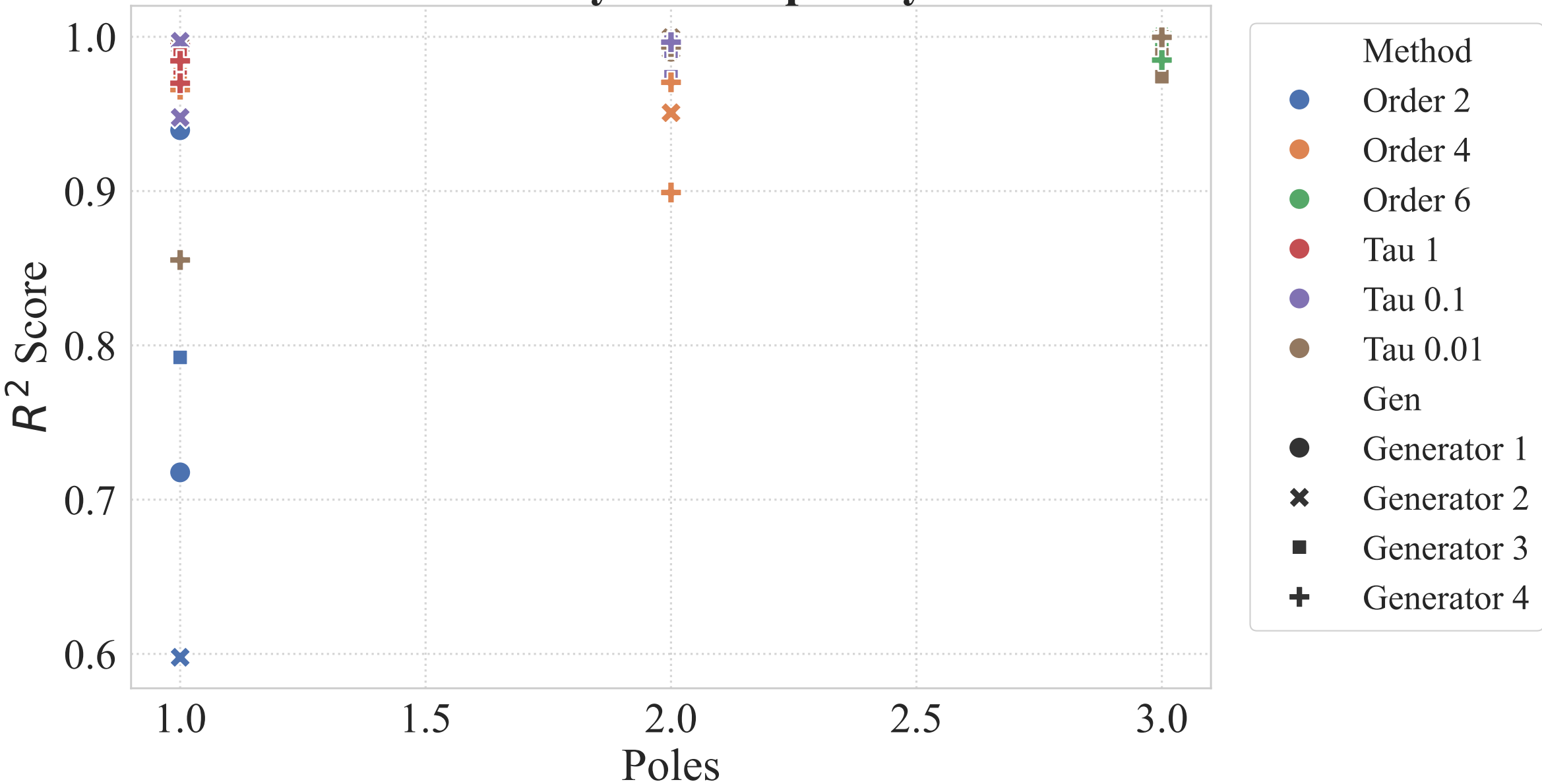
Accuracy vs Complexity
