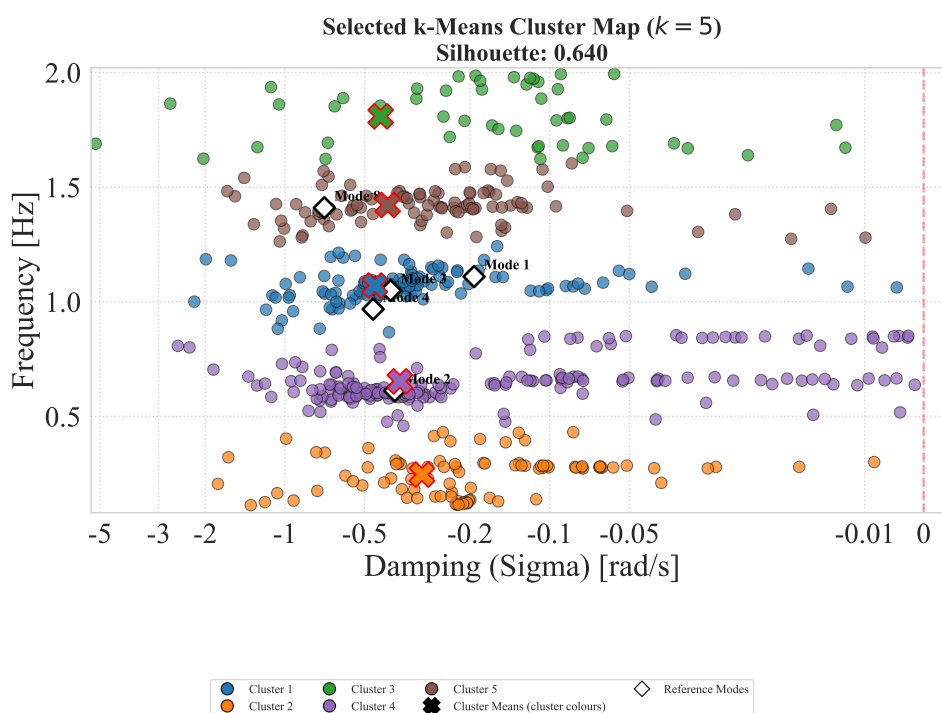
Σχήμα Β'.1: Selected cluster map: k-Means (orders1).
