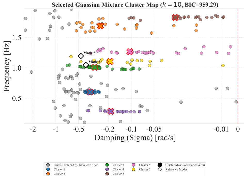
Σχήμα Β'.13: Selected cluster map: GMM (orders1).
