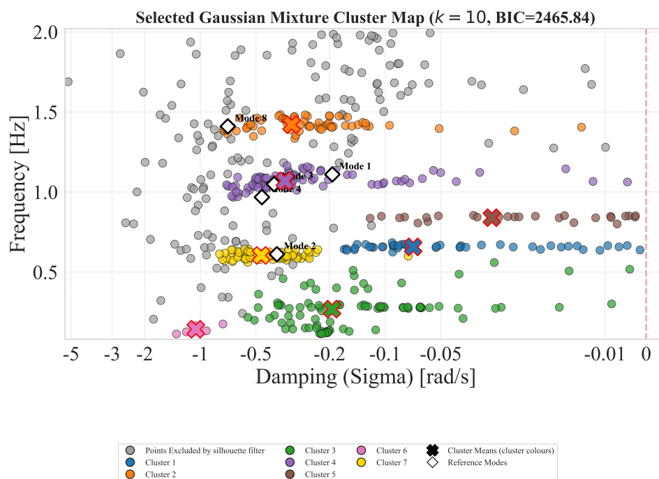
Σχήμα Β'.6: Selected cluster map: GMM (orders1).
