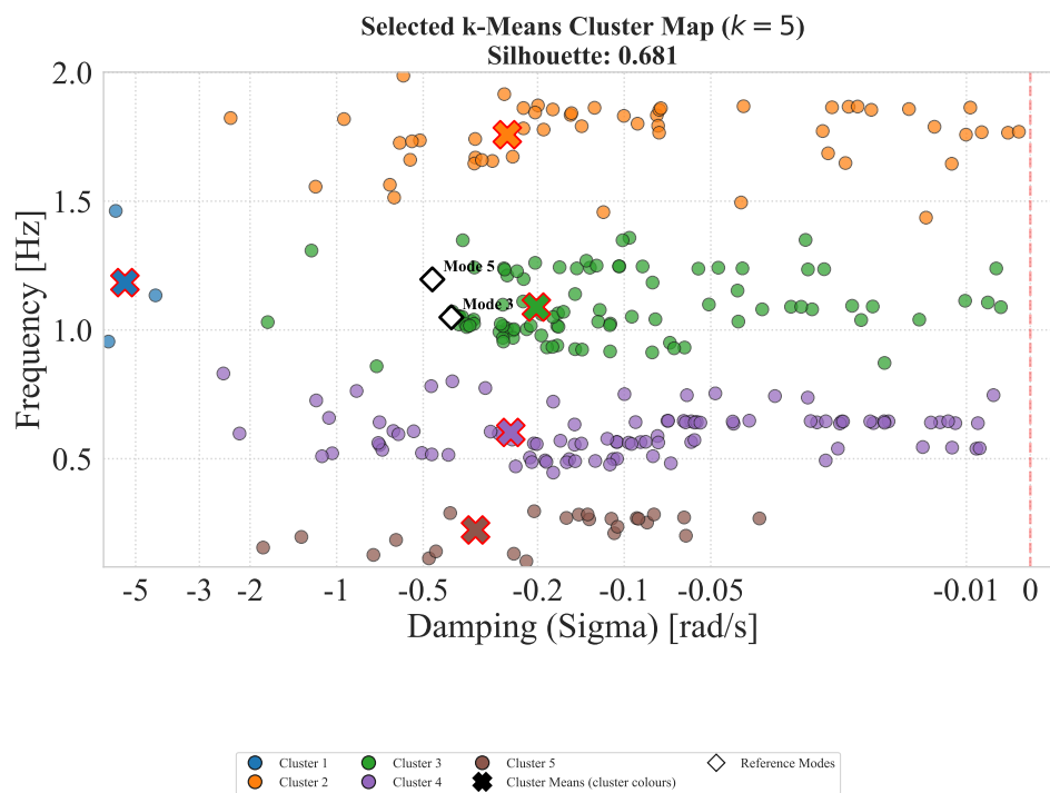
Σχήμα Β'.29: Selected cluster map: k -Means (orders2).
