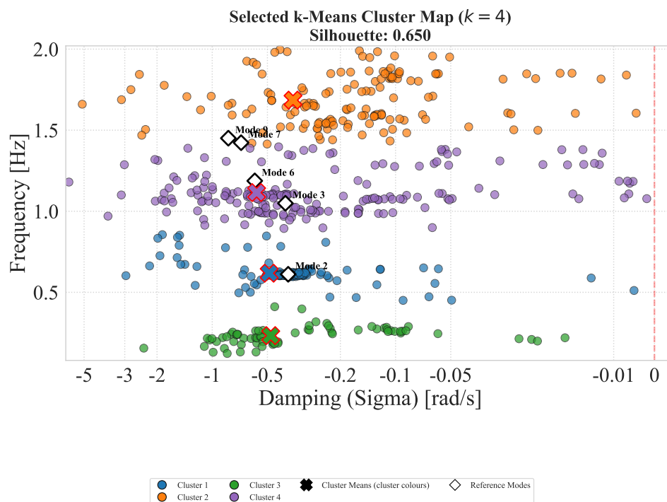
Σχήμα Β'.15: Selected cluster map: k-Means (orders1).
