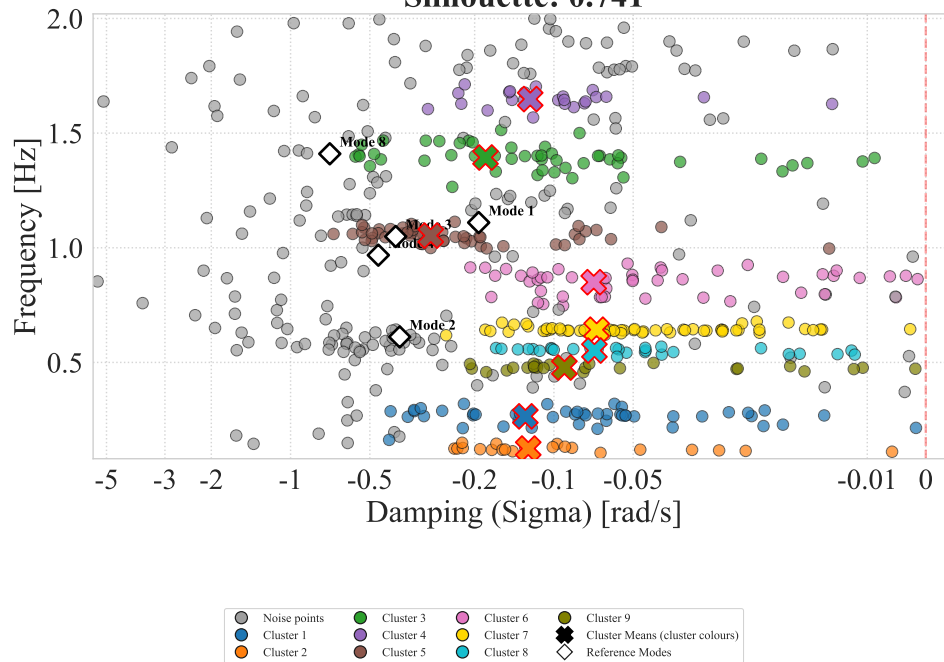
Selected HDBSCAN Cluster Map ( \min\_cluster\_size = 20, \varepsilon = 0.06 ): Silhouette: 0.741
