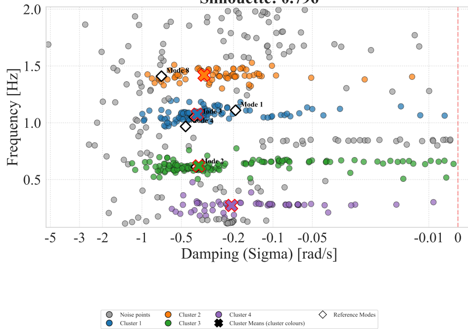
Σχήμα Α'.5: Selected cluster map: HDBSCAN (orders1).
