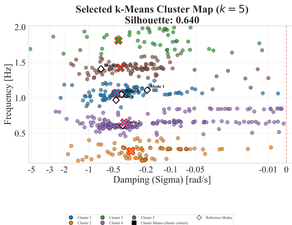
Σχήμα Α'.1: Selected cluster map: k-Means (orders1).
