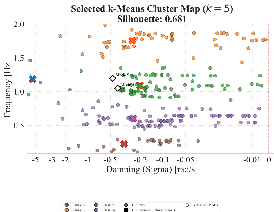
Σχήμα Α'.29: Selected cluster map: k-Means (orders2).
