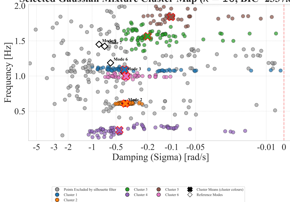
Σχήμα Α'.20: Selected cluster map: GMM (orders1).
