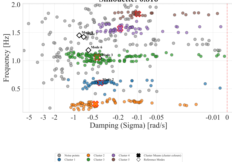
Σχήμα Α'.19: Selected cluster map: HDBSCAN (orders1).
