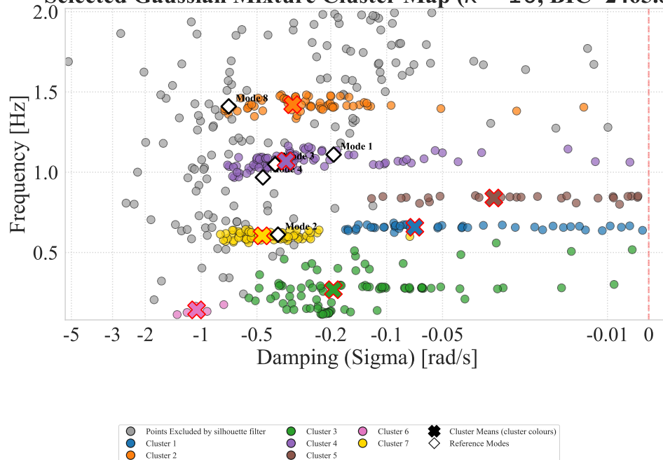
Σχήμα Α'.6: Selected cluster map: GMM (orders1).
