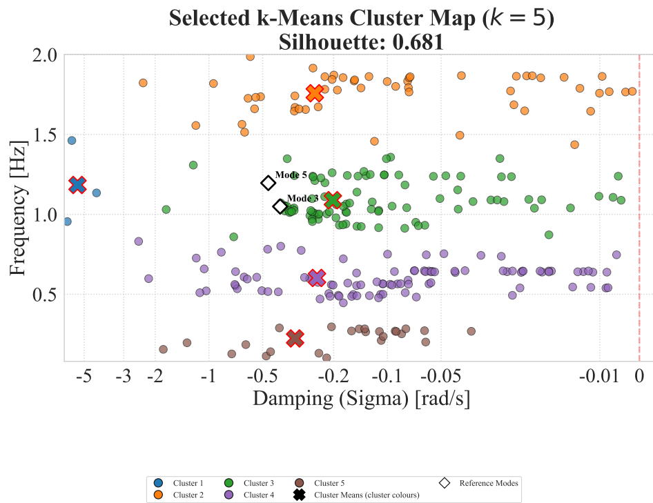
Σχήμα Α'.29: Selected cluster map: k -Means (orders2).
