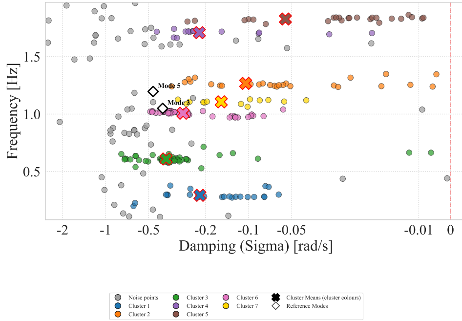
Selected HDBSCAN Cluster Map ( \text{min\_cluster\_size} = 12, \varepsilon = 0.06 ): Silhouette: 0.782
