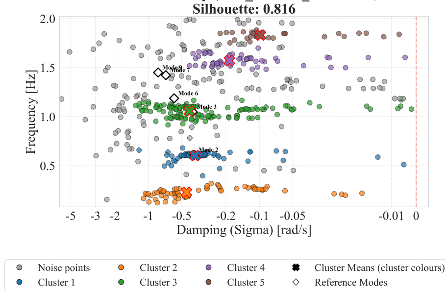
Selected HDBSCAN Cluster Map ( min\_cluster\_size = 24, \epsilon = 0.061, eom )
