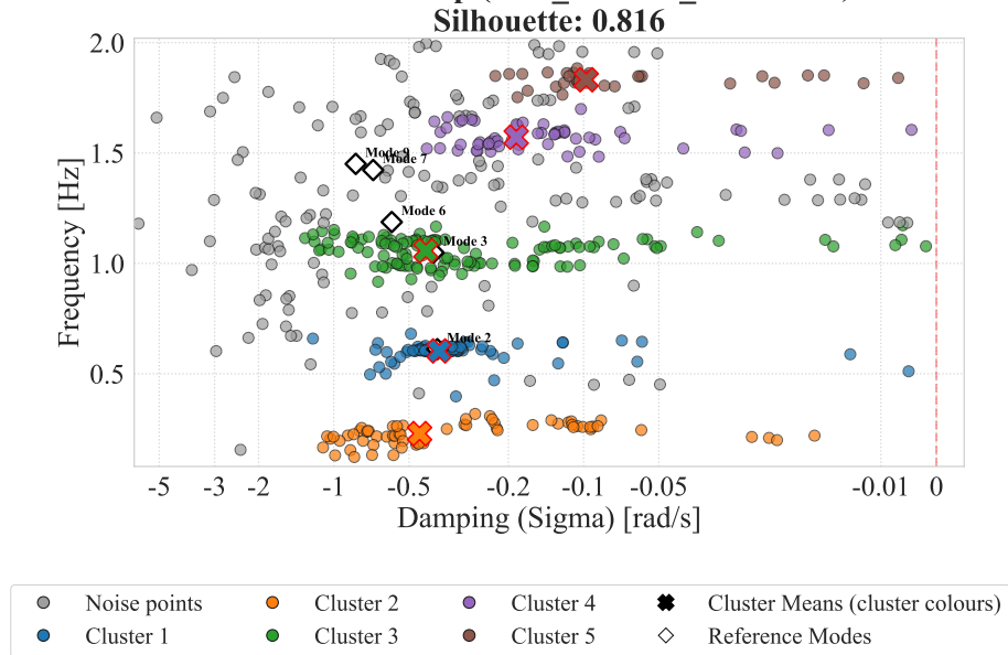
Selected HDBSCAN Cluster Map ( \min\_cluster\_size = 24, \varepsilon = 0.061, eom )
