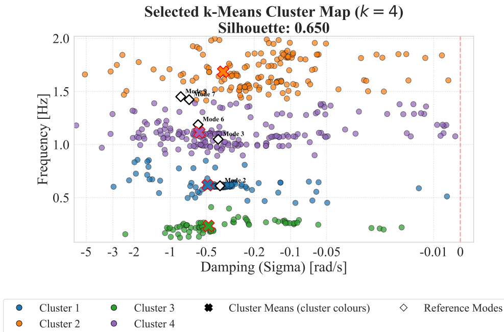
Σχήμα Α'.15: Selected cluster map: k-Means (orders1).
