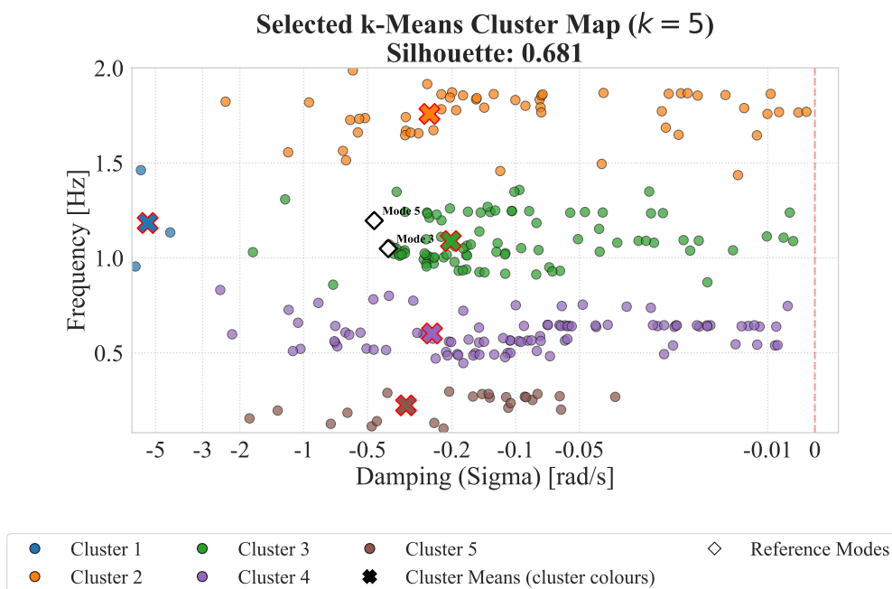
Σχήμα Α'.29: Selected cluster map: k-Means (orders2).
