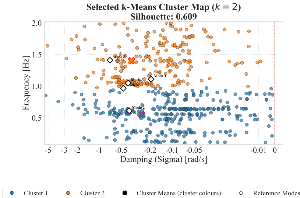
Σχήμα Α'.22: Selected cluster map: k-Means (orders2).
