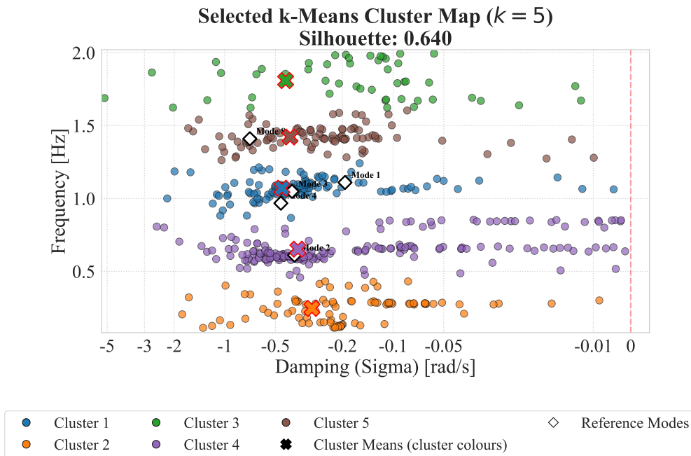
Σχήμα Α'.1: Selected cluster map: k-Means (orders1).
