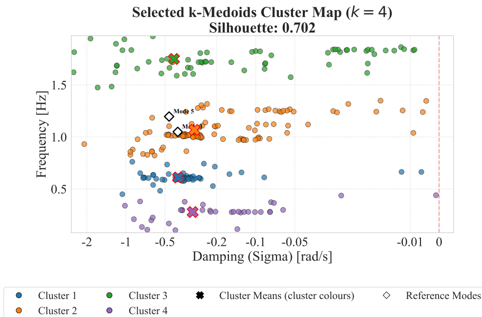
Σχήμα Α'9: Selected cluster map: k-Medoids (orders1).
