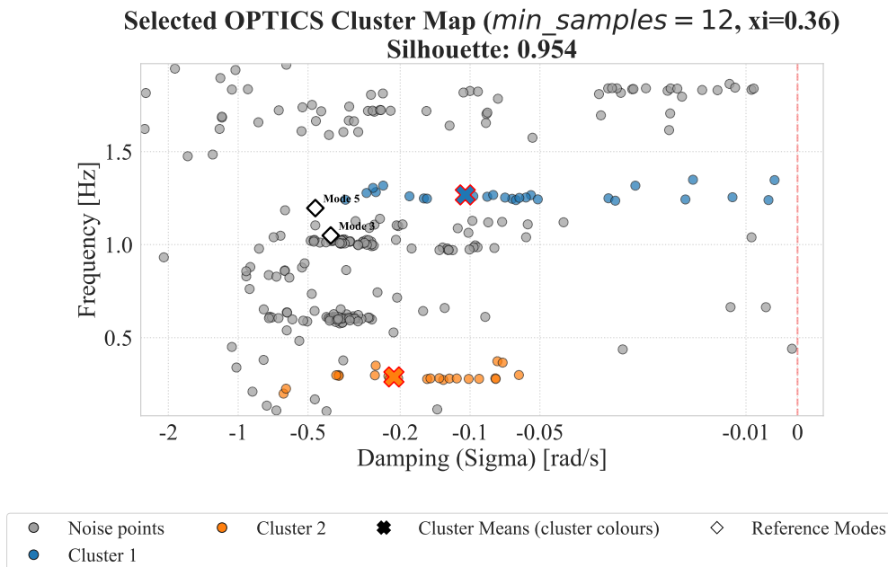
Σχήμα Α'.11: Selected cluster map: OPTICS (orders1).
