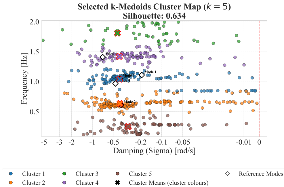
Σχήμα Α'.2: Selected cluster map: k-Medoids (orders1).
