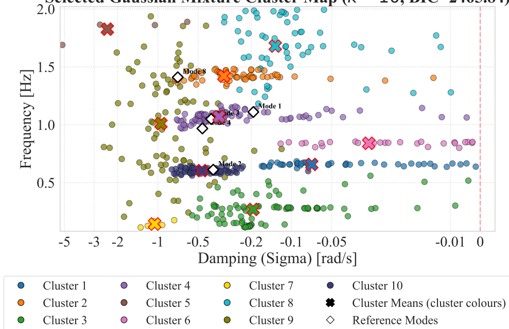
Σχήμα Α'.6: Selected cluster map: GMM (orders1).
