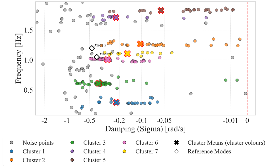
Σχήμα Α'.12: Selected cluster map: HDBSCAN (orders1).
