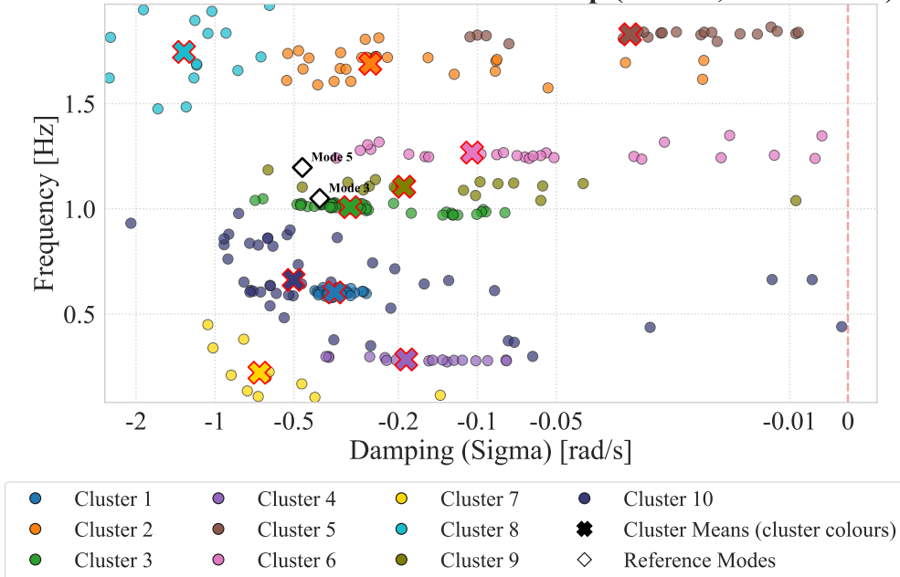
Selected Gaussian Mixture Cluster Map ( k = 10, BIC=959.29 )
