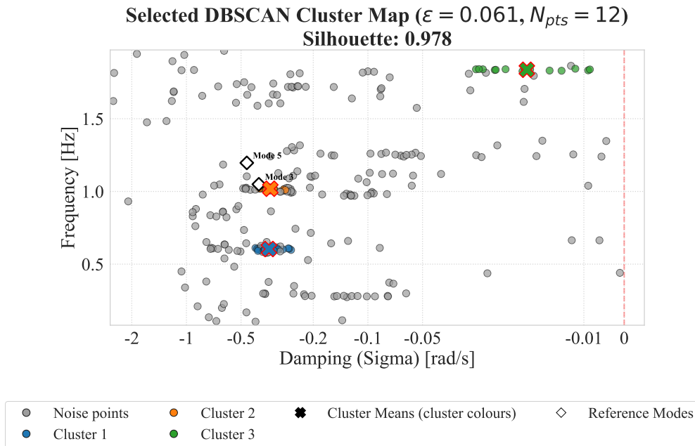
Σχήμα Α'.10: Selected cluster map: DBSCAN (orders1).
