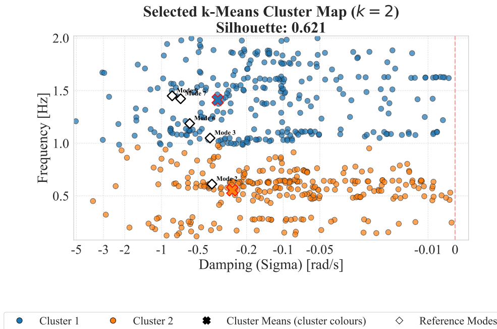
Σχήμα Α'.36: Selected cluster map: k-Means (orders2).
