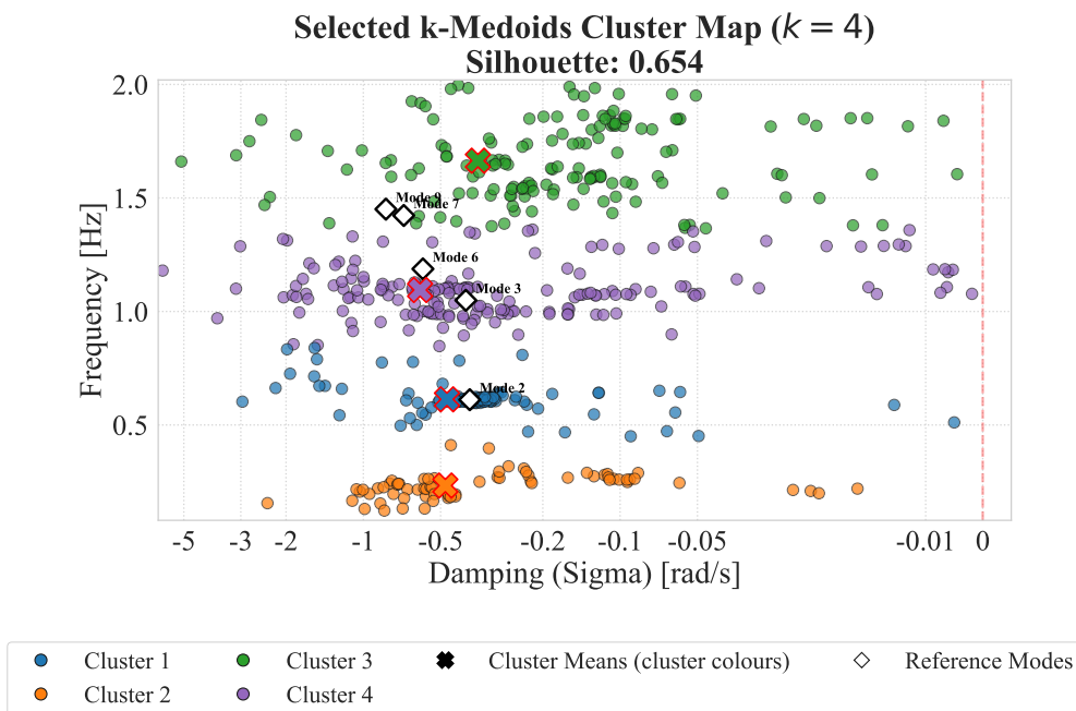
Σχήμα Α'.16: Selected cluster map: k-Medoids (orders1).
