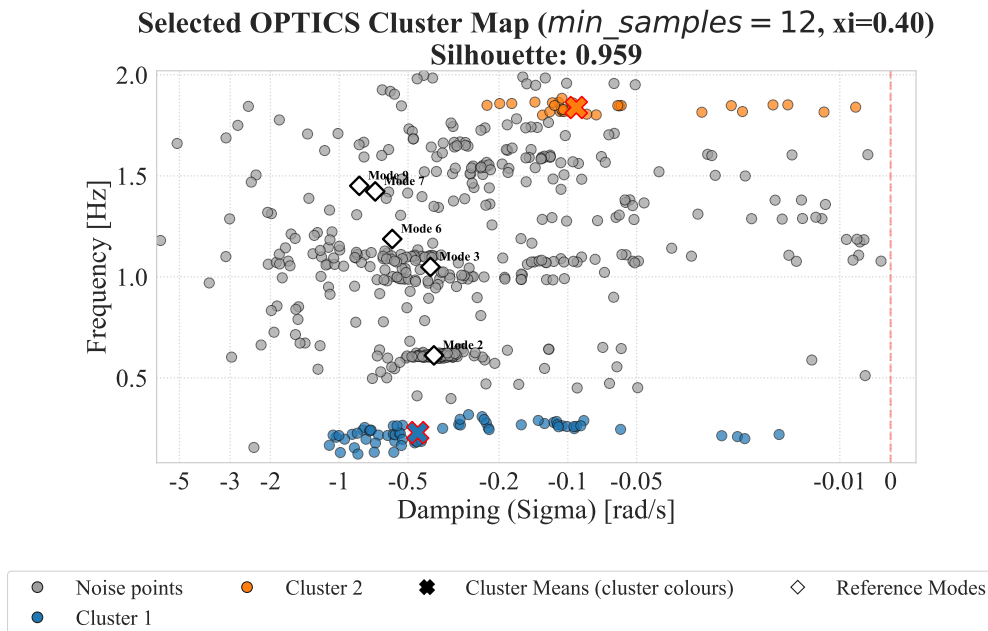
Σχήμα Α'.18: Selected cluster map: OPTICS (orders1).
