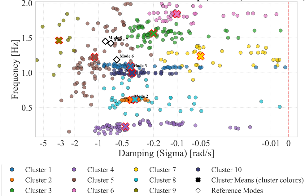
Selected Gaussian Mixture Cluster Map ( k = 10, BIC=2337.83 )
