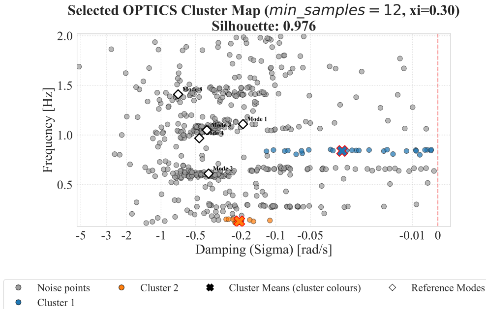
Σχήμα Α'.4: Selected cluster map: OPTICS (orders1).
