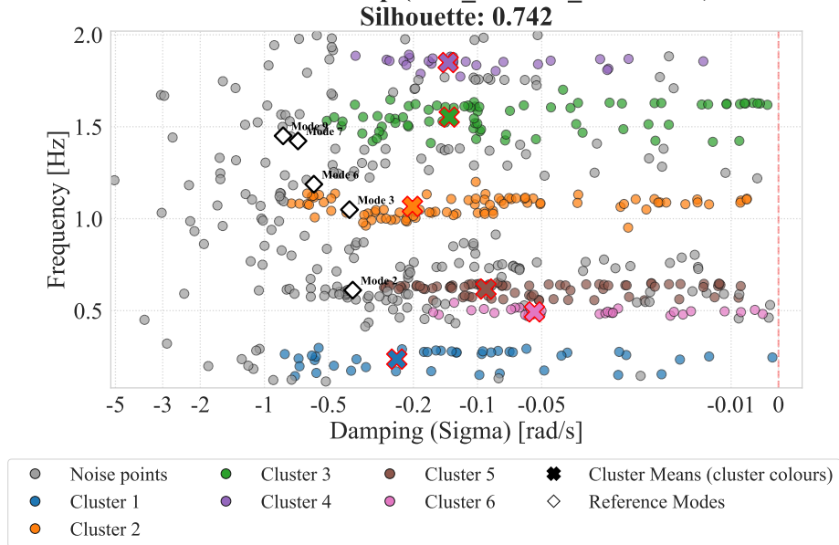
Selected HDBSCAN Cluster Map ( \min\_cluster\_size = 26, \epsilon = 0.061, \text{leaf} )
