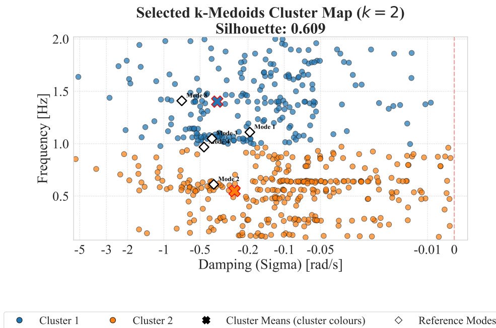
Σχήμα Α'.23: Selected cluster map: k-Medoids (orders2).
