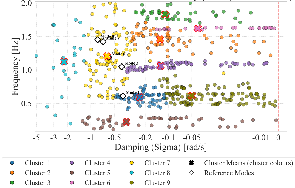
Selected Gaussian Mixture Cluster Map ( k = 9, \text{BIC}=2559.48 )
