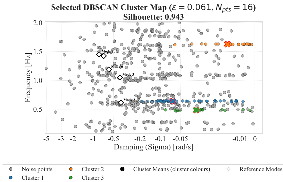
Σχήμα Α'.38: Selected cluster map: DBSCAN (orders2).
