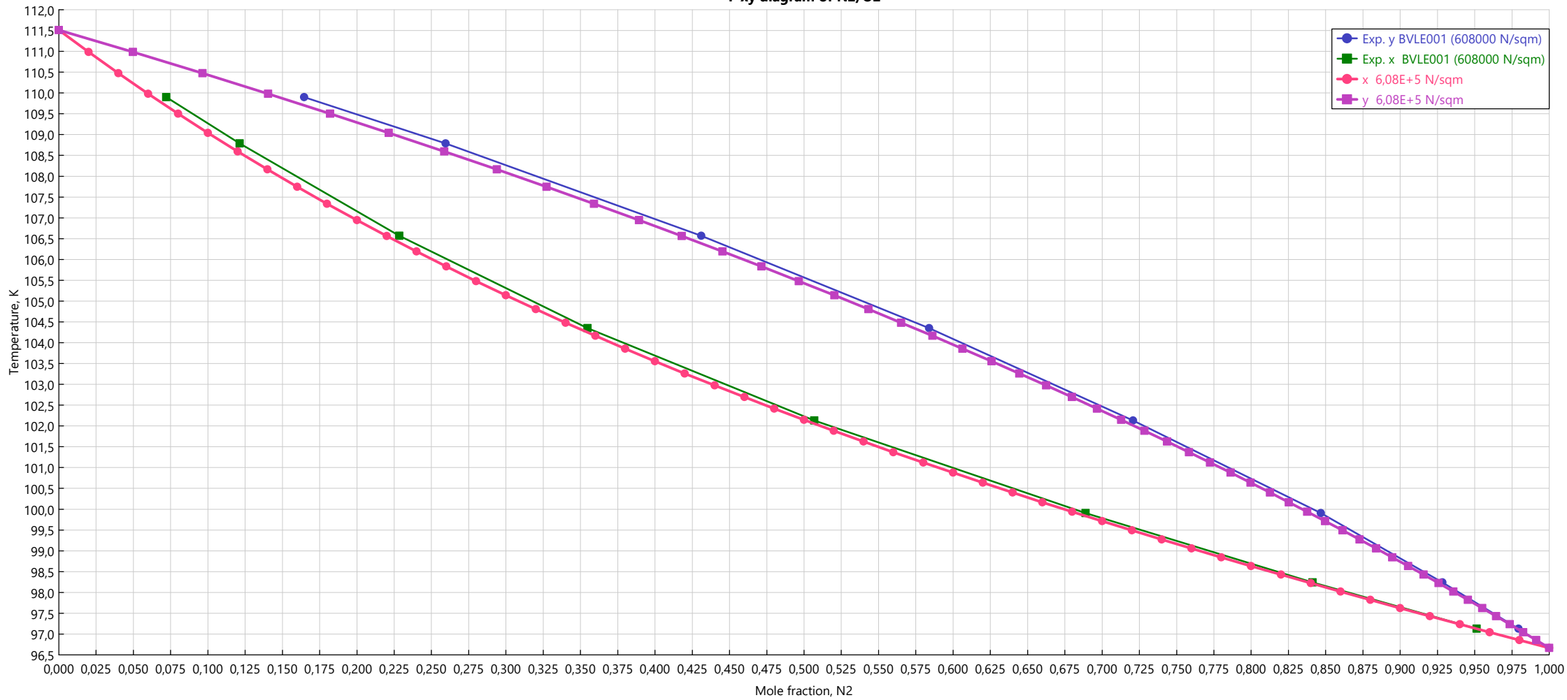
T-xy diagram of N2/O2
