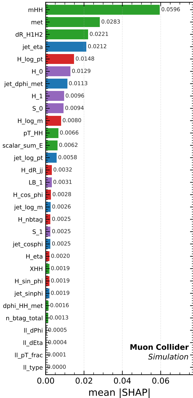
(a) \sqrt{s} = 3 \text{ TeV}
