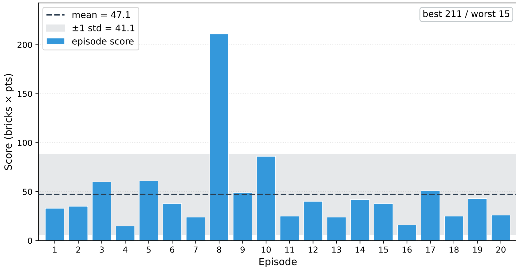
Breakout episode scores — baseline (ball-tracking) (n = 20)
