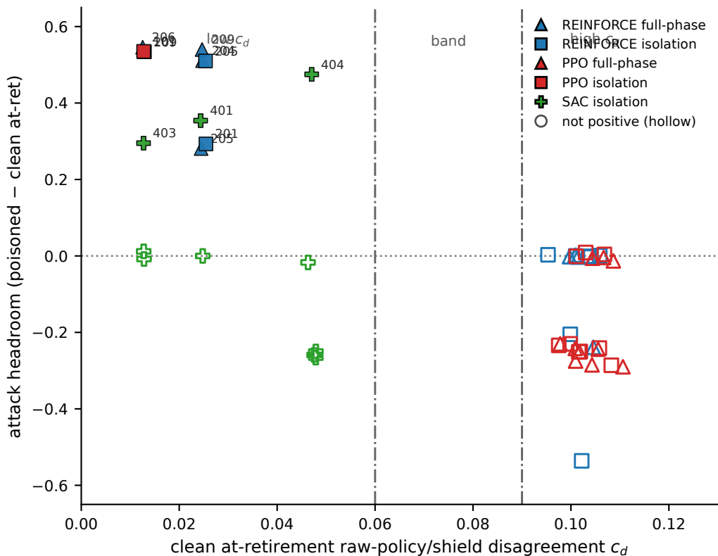
Attack headroom vs. clean retirement-state disagreement ( n = 50 )
