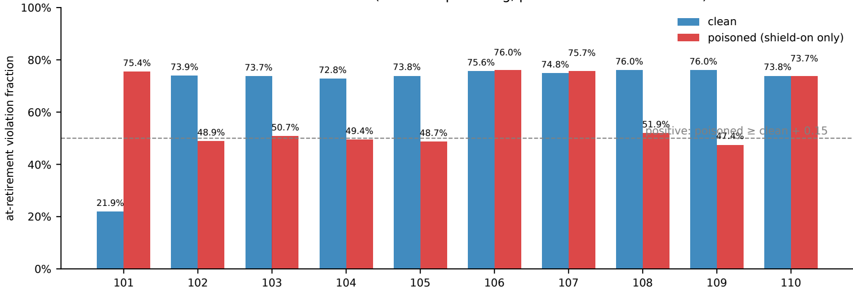
PPO retirement isolation (shield-on poisoning, paired run indices 101-110)
