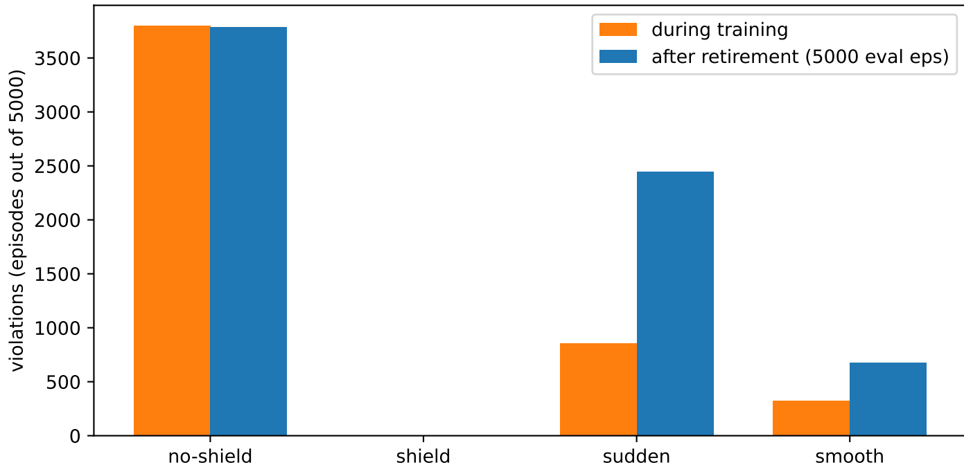
Clean baseline (obstacle, REINFORCE, seed 1) — paper Tab. 1 protocol
